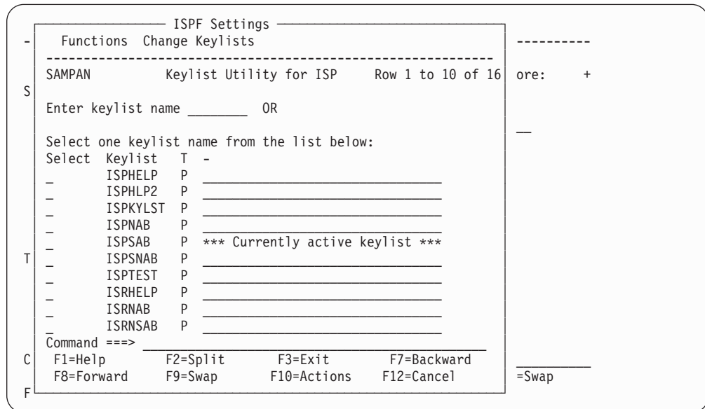
Figure 35. Sample CUA panel (SAMPAN on ISPKLUP)
