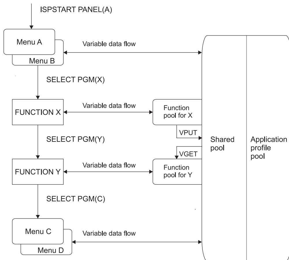
Figure 21. Control and data flow in a dialog
