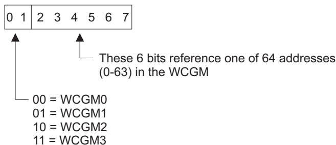
Figure 34. Character Arrangement Table Module Structure
