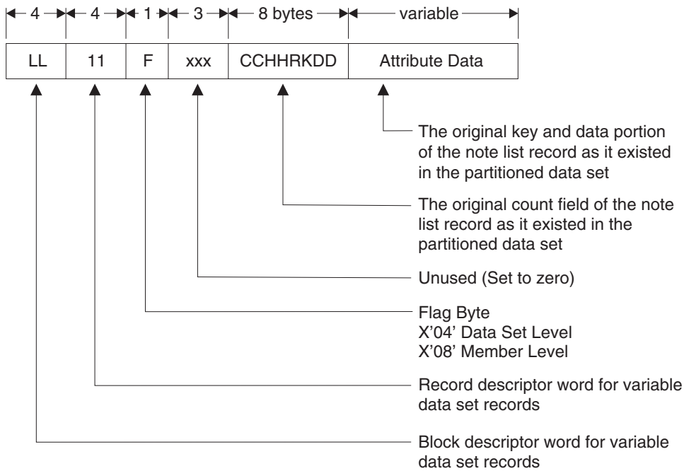
Figure 50. Attribute Record Layout
