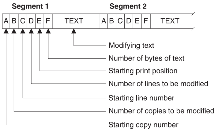
Figure 32. Copy Modification Module Structure
