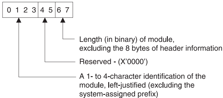
Figure 26. 3800 General Module Header
