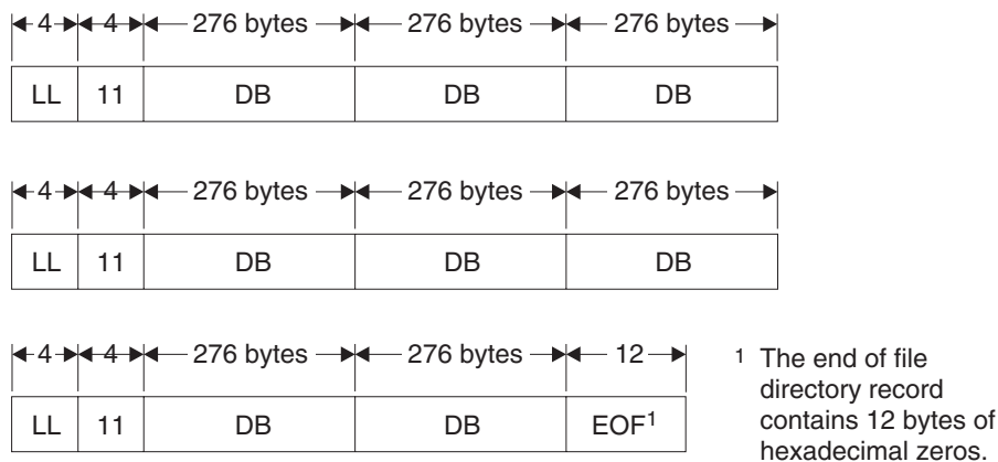
Figure 49. Directory Record Layout
