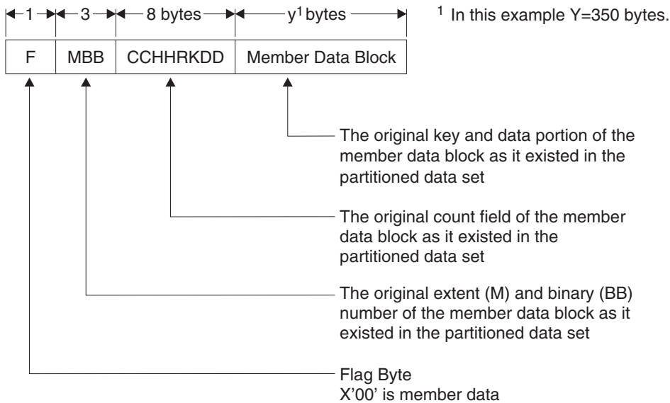
Figure 53. Member Data Block Layout
