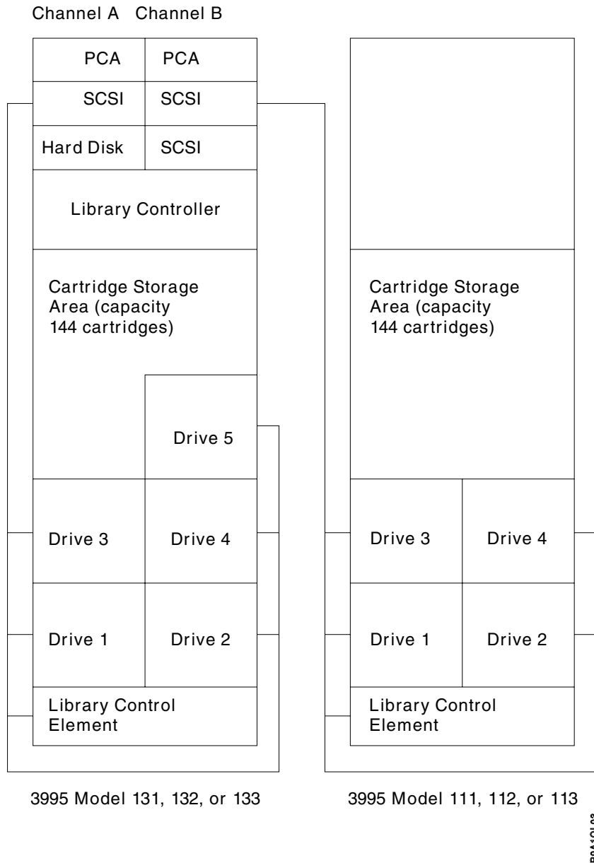
Figure 32. Sample Hardware Configuration—IBM 3995 Models 131, 132, 133, 111, 112, 113
