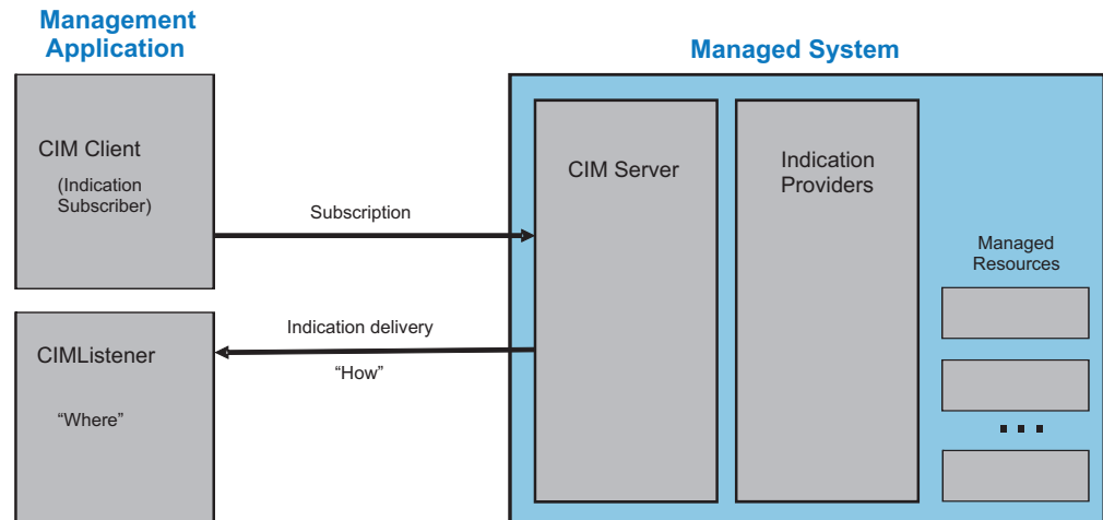
Figure 20. Indication Handler
