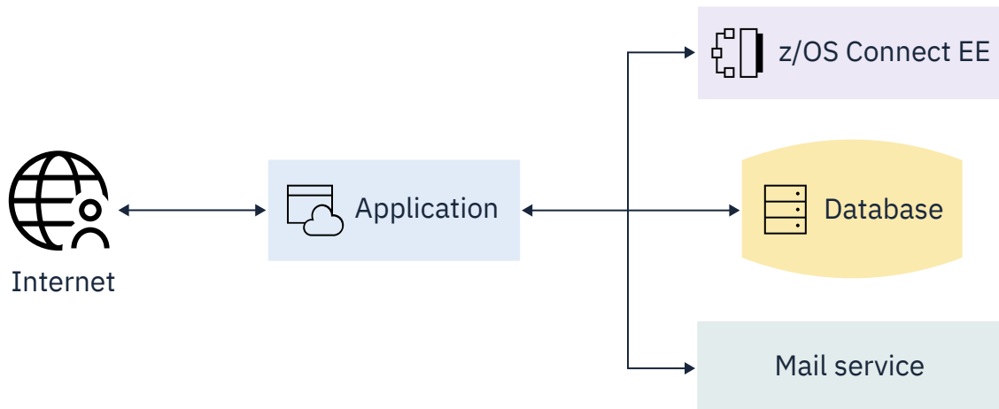
Figure 5. Backing services
