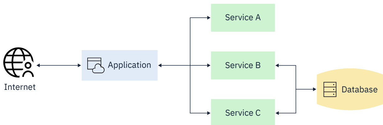
Figure 6. Hosted services
