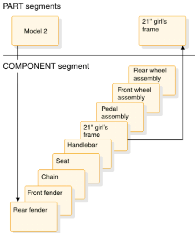
Figure 91. Extra database records required for the Model 2 bicycle
