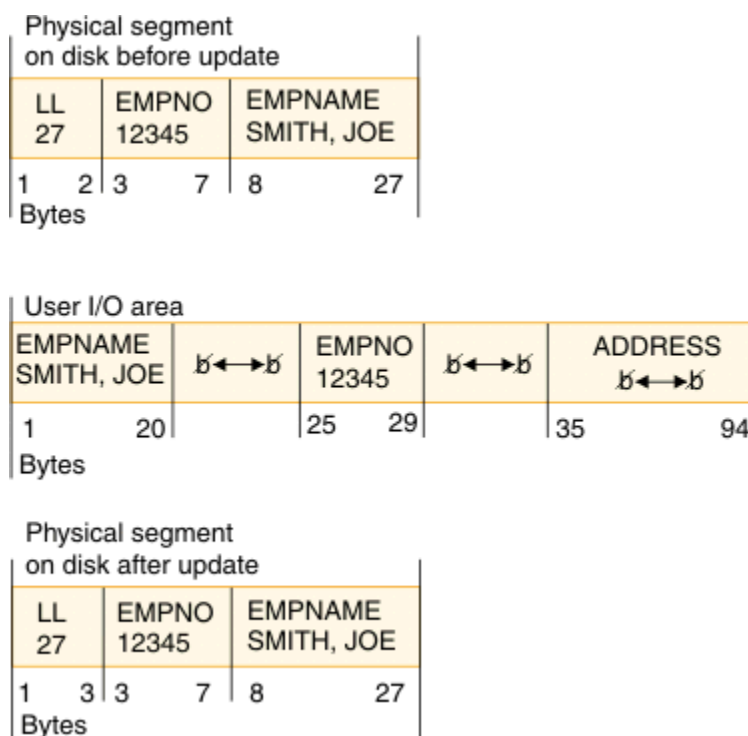
Figure 204. First example of a missing field on a replace call
