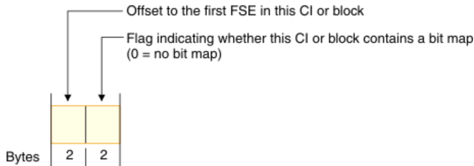
Figure 47. An FSEAP
