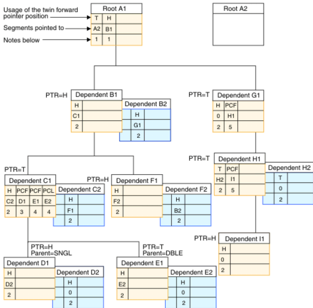
Figure 44. Mixing pointers
