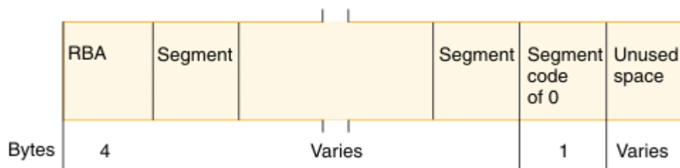
Figure 26. Format of a logical record in a HISAM database
