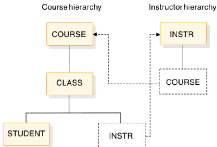
Figure 222. Bidirectional logical relationships
