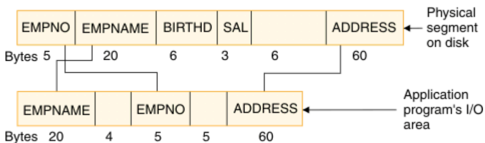
Figure 199. DBD and PSB coding for field-level sensitivity
