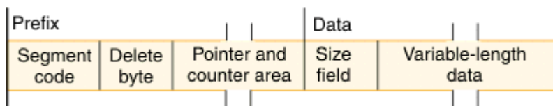
Figure 197. Format of HISAM variable-length segments
