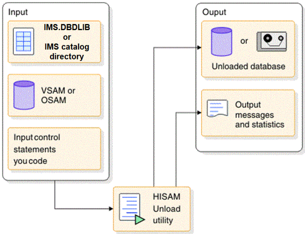
Figure 250. HISAM Reorganization Unload utility (DFSURUL0)
