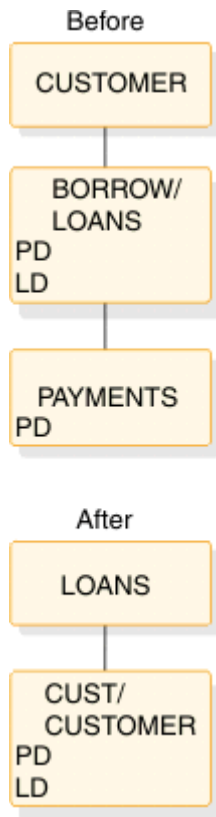
Figure 153. Logical child, physical pairing—virtual delete rule example: before and after
