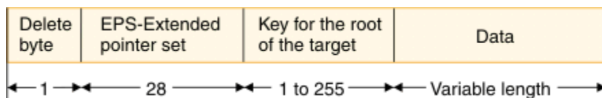
Figure 181. Secondary index entry for HALDB
