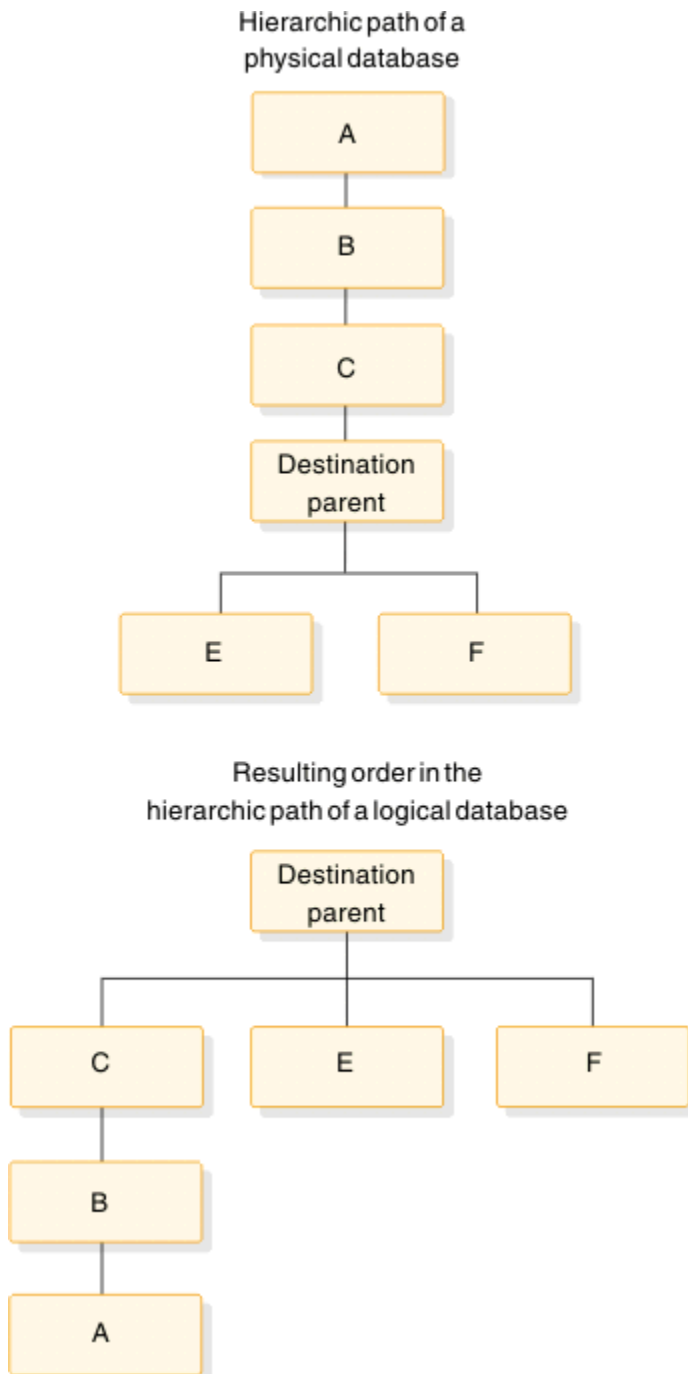
Figure 98. Logical database hierarchy enabled by crossing the first logical relationship
