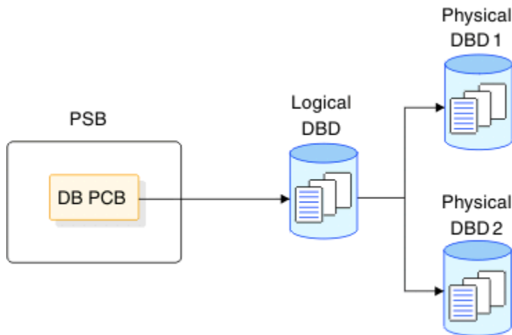
Figure 92. Relationship of control blocks when a logical relationship is used
