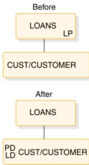
Figure 119. Logical parent, physical pairing—physical delete rule example: before and after
