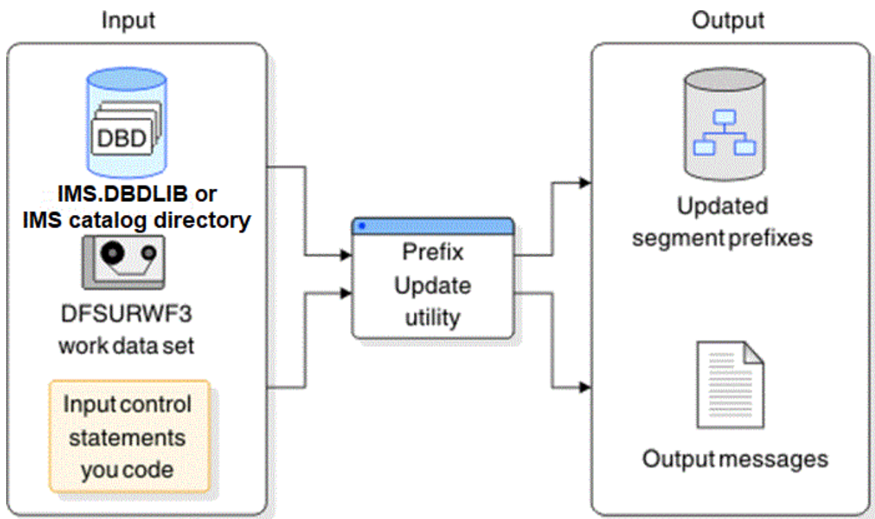
Figure 257. Database Prefix Update utility (DFSURGP0)
