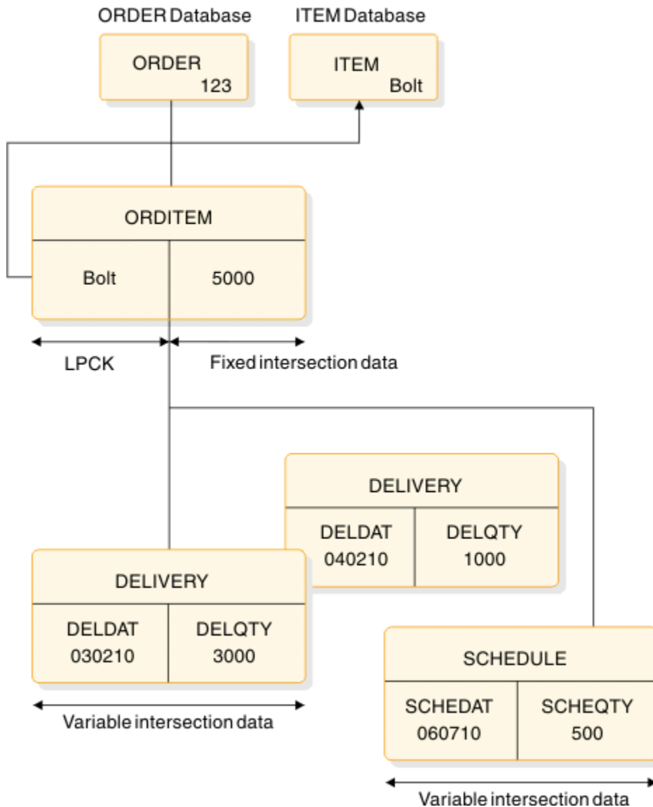
Figure 88. Variable intersection data
