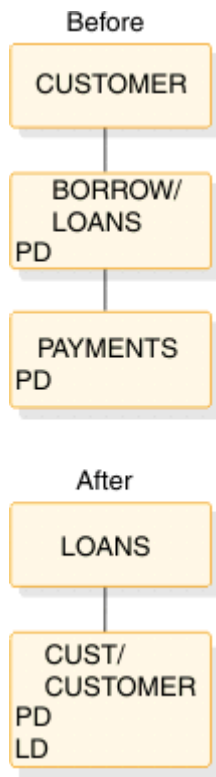
Figure 144. Logical child, virtual pairing—logical delete rule example: before and after
