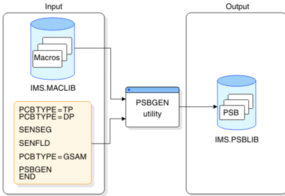
Figure 233. The PSB generation process
