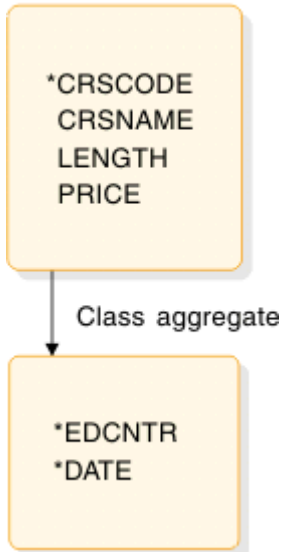
Figure 217. Schedule of classes conceptual data structure
