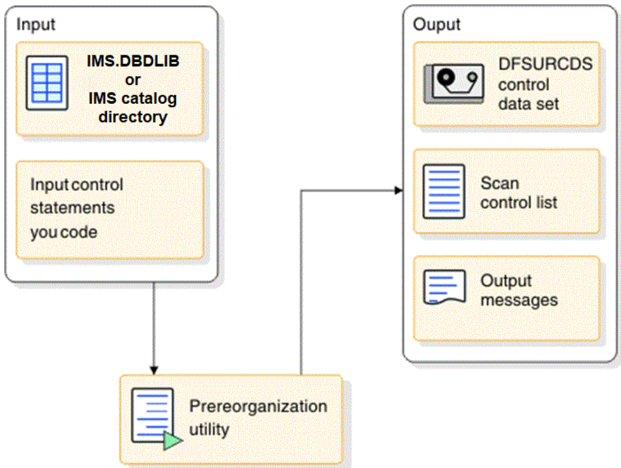
Figure 254. Database Prereorganization utility (DFSURPRO)
