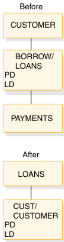
Figure 150. Logical child, virtual pairing—virtual delete rule example: before and after
