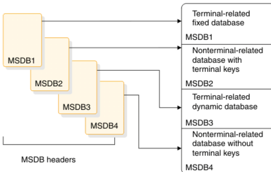
Figure 66. MSDB pointers
