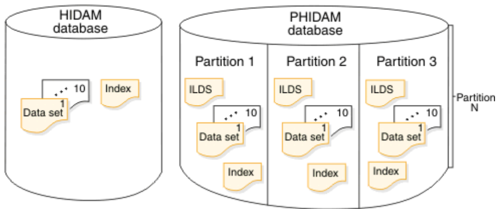
Figure 34. A comparison of the logical views of HIDAM and PHIDAM databases
