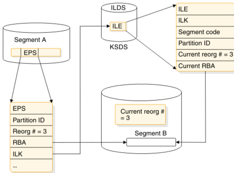
Figure 83. Self-healing pointers
