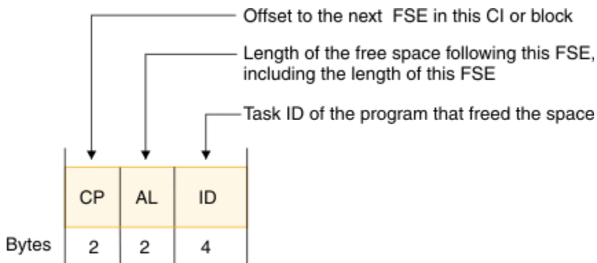
Figure 48. An FSE
