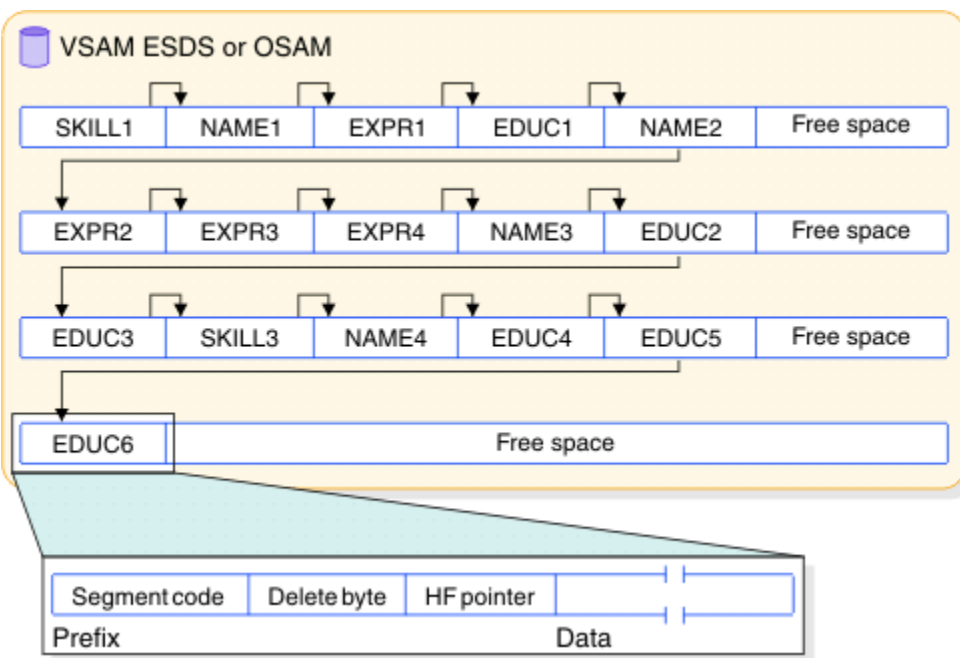
Figure 52. HIDAM database records in storage
