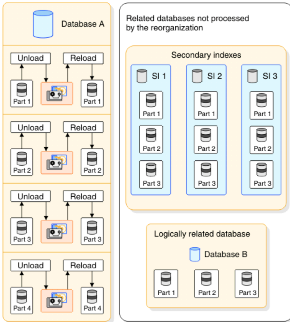
Figure 262. Offline reorganization of a HALDB database
