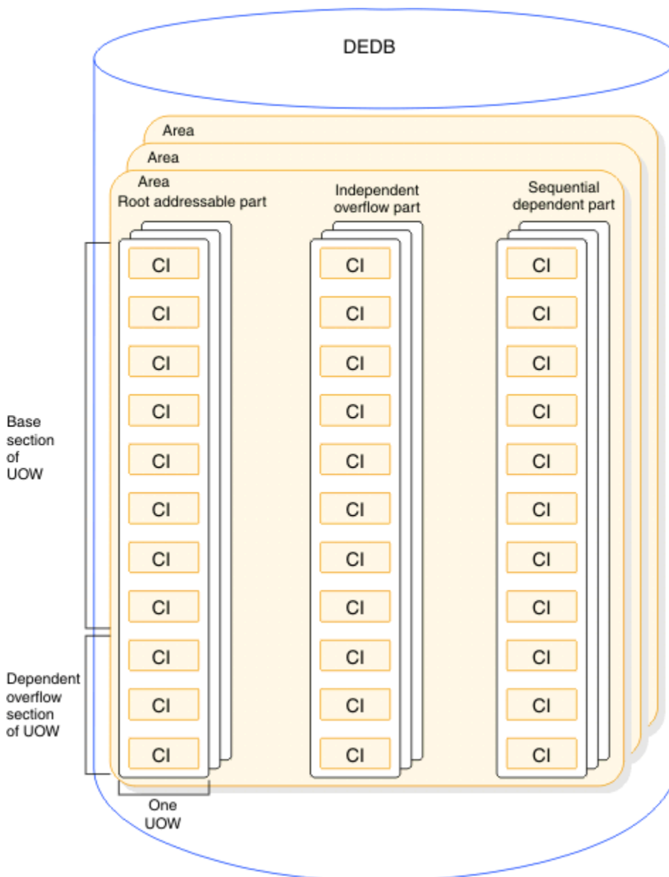
Figure 59. Parts of a DEDB area in storage
