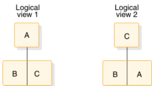
Figure 111. Logical views for replace rules table
