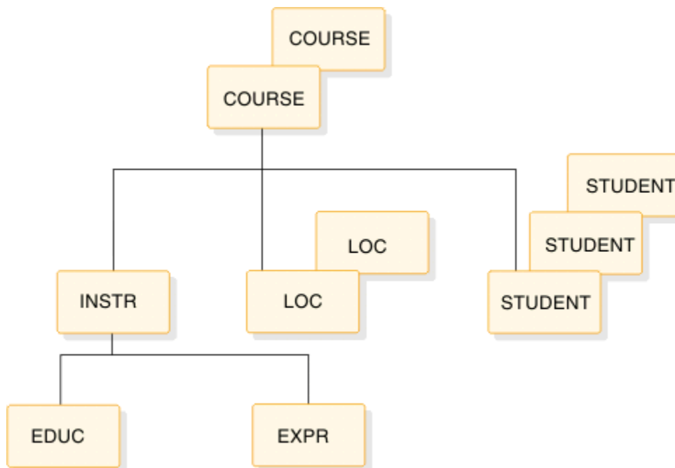
Figure 36. Example database record for illustrating pointers
