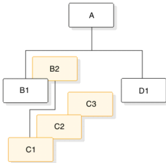
Figure 31. The hierarchical segment layout on the database
