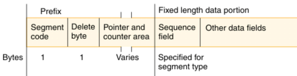
Figure 9. Format of fixed-length segments
