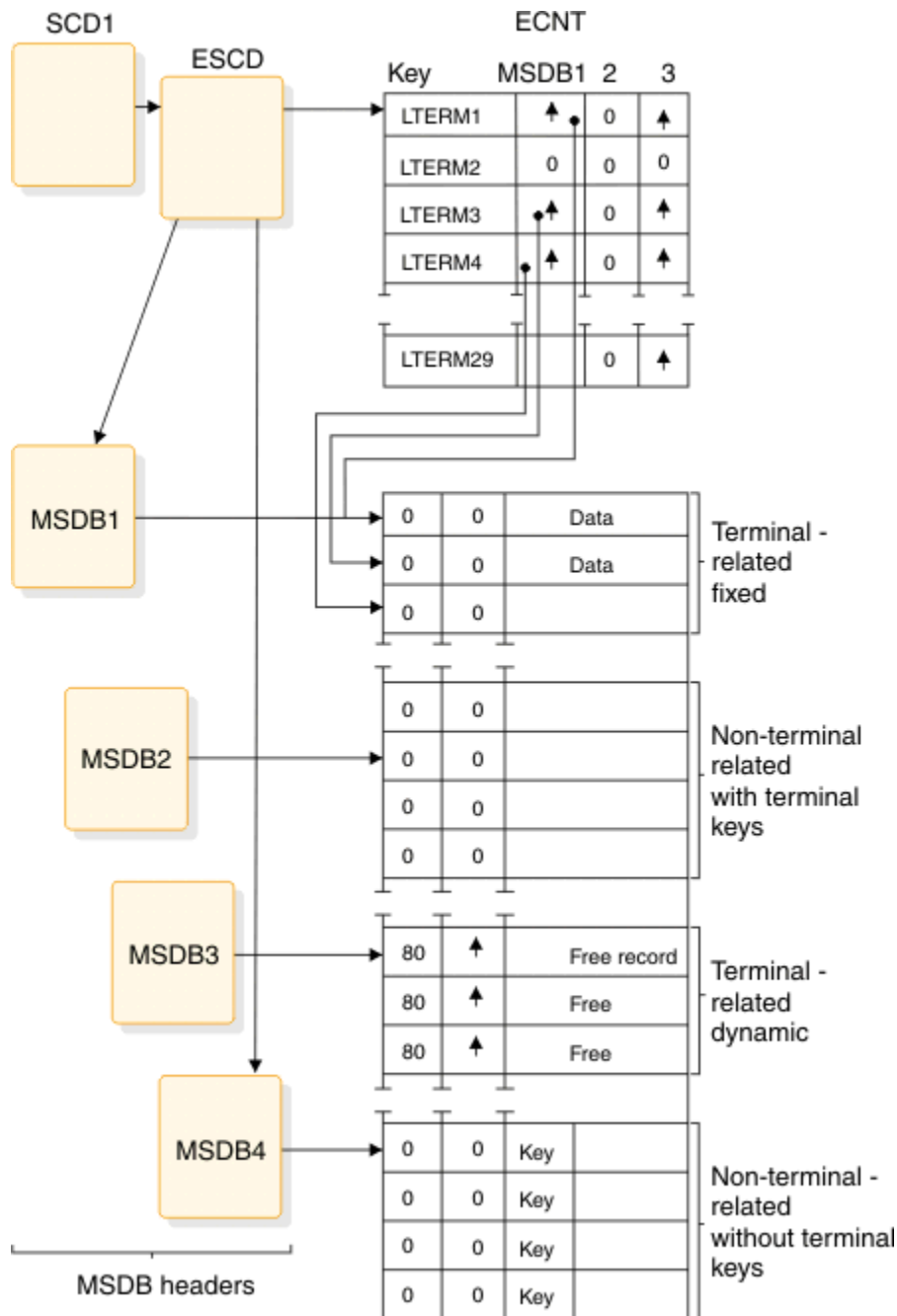
Figure 69. ECNT and MSDB storage layout
