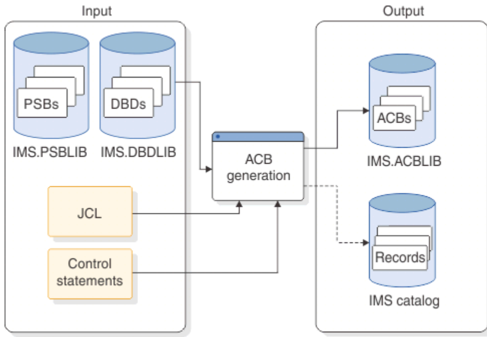
Figure 235. The ACB generation process
