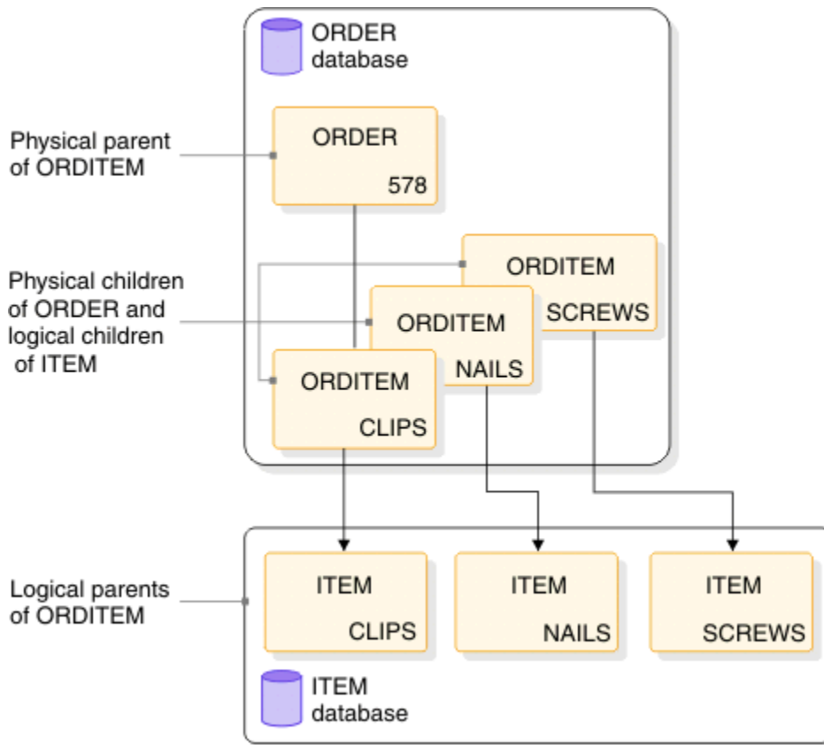
Figure 74. Unidirectional logical relationship
