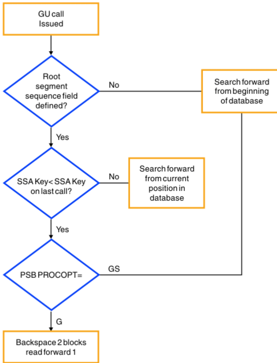
Figure 22. GU calls against an HSAM database
