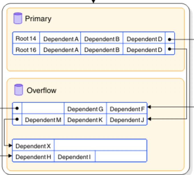
Figure 30. Inserting a dependent segment into a HISAM database (no space exists in the logical record)
