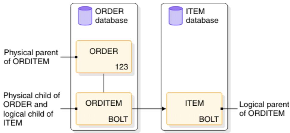
Figure 70. A simple logical relationship
