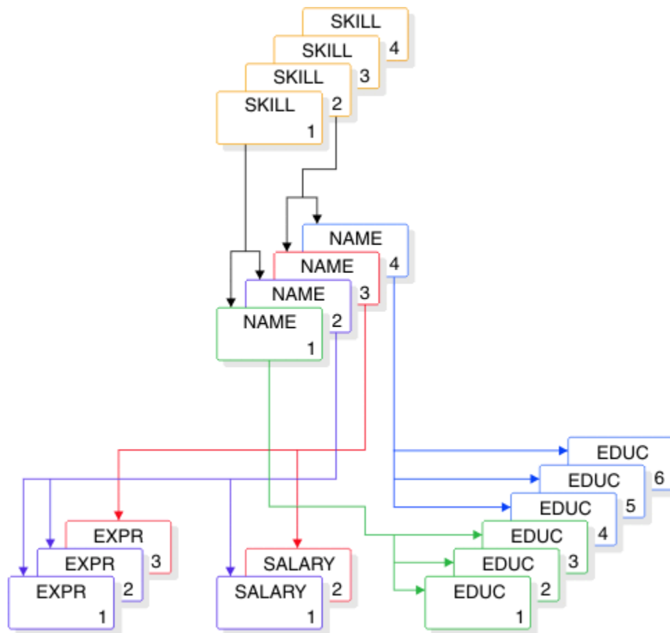
Figure 24. Example HISAM database records
