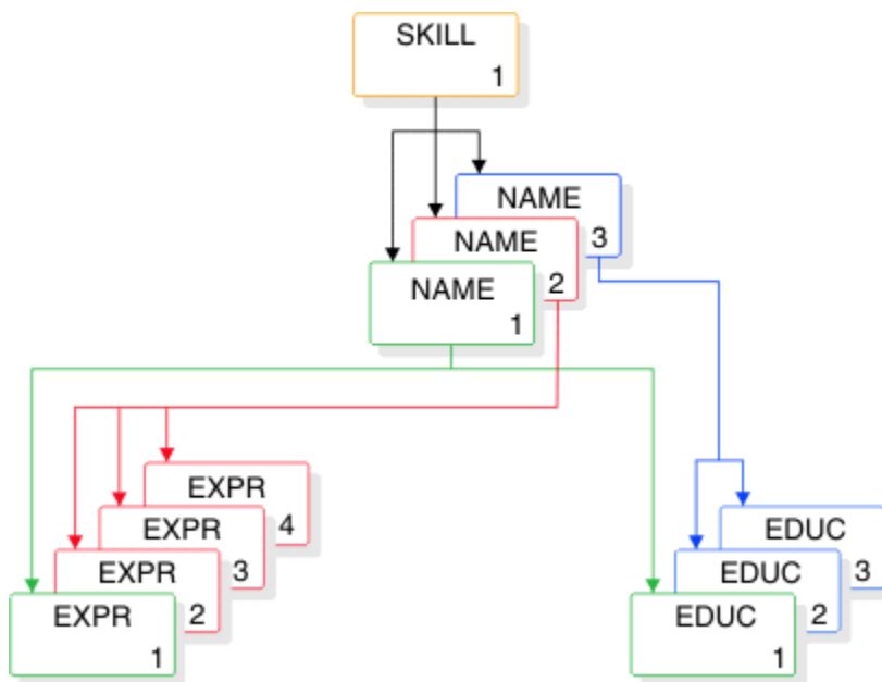
Figure 20. Example HSAM database
