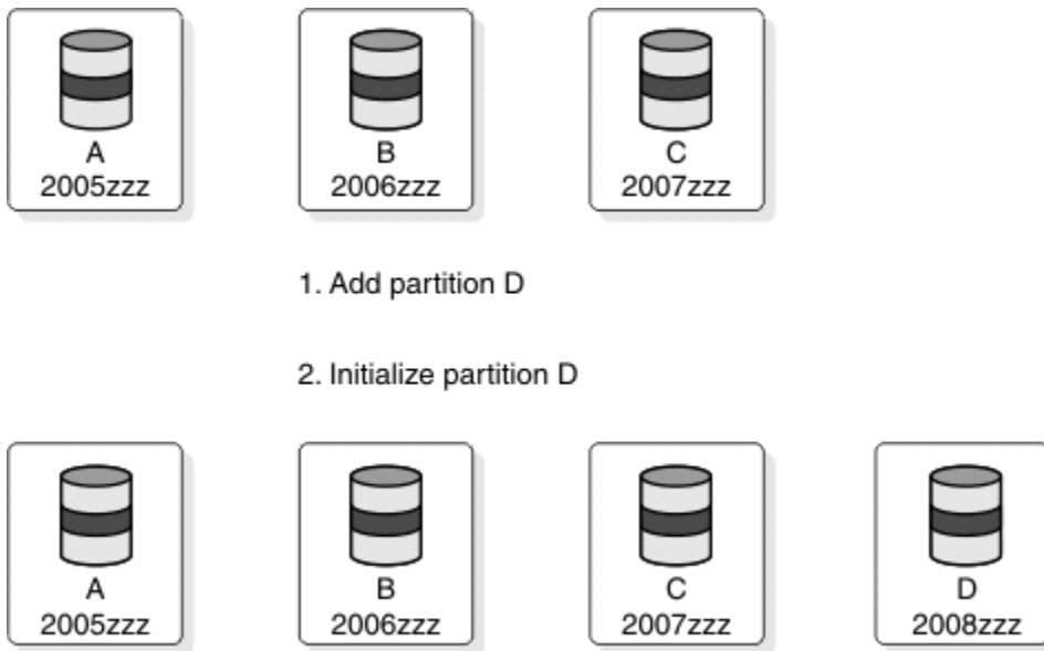
Figure 295. Adding a higher key partition with key range partitioning
