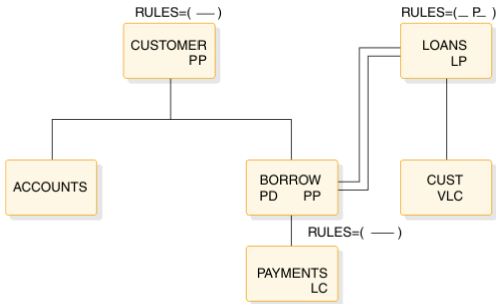
Figure 118. Logical parent, virtual pairing—physical delete rule example
