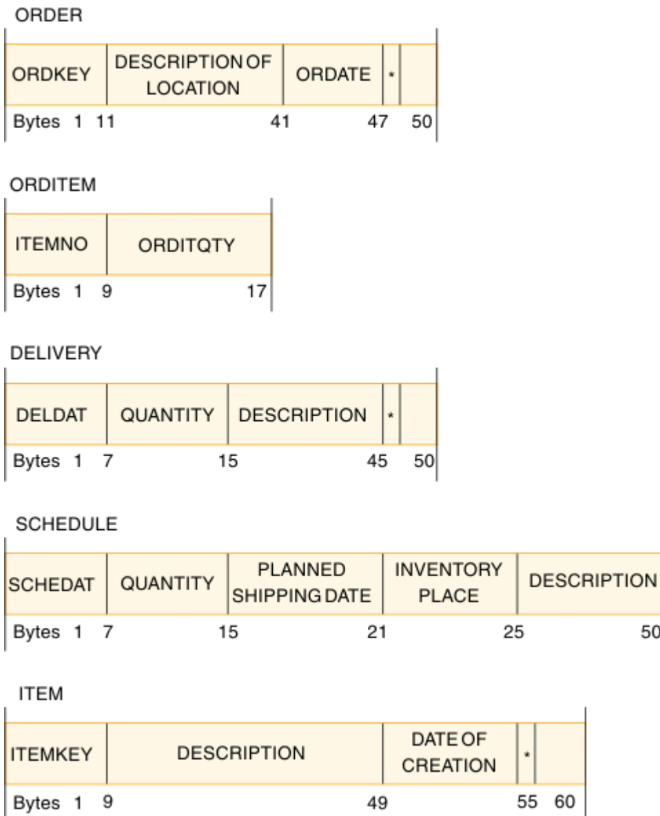
Figure 93. Layouts of segments used in the examples
