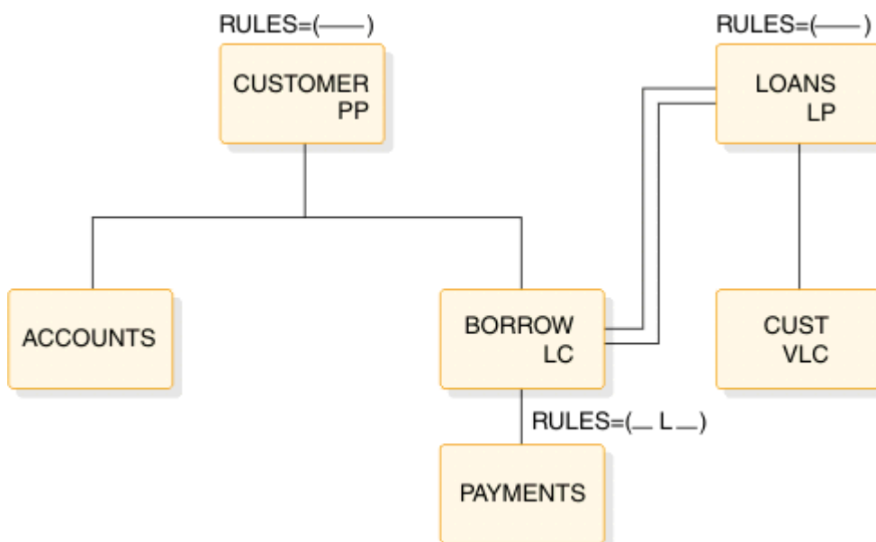
Figure 142. Logical child, virtual pairing—logical delete rule example
