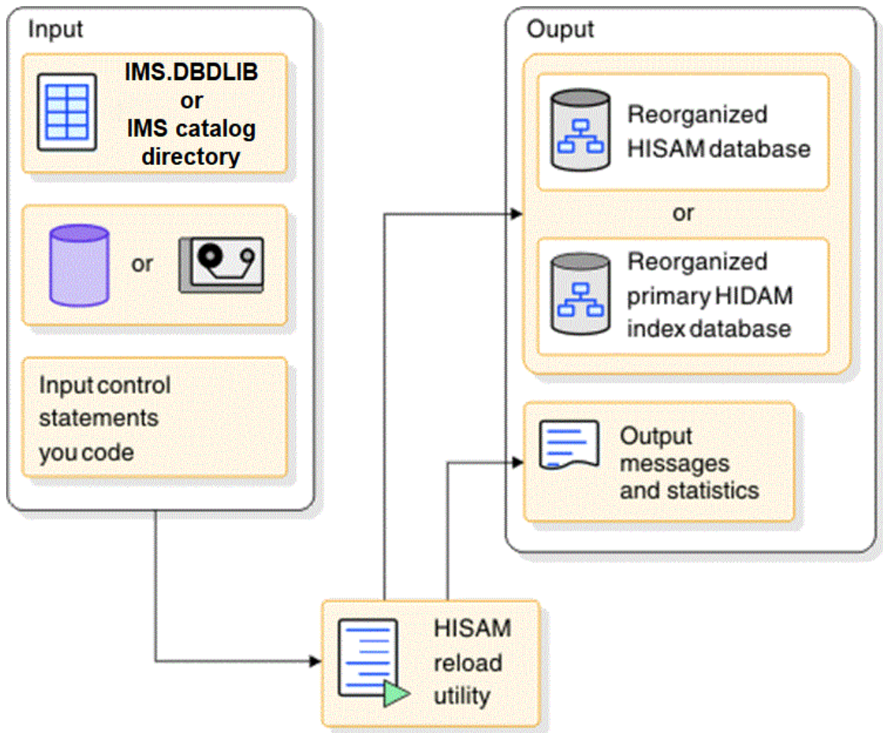
Figure 251. HISAM Reorganization Reload utility (DFSURRL0)
