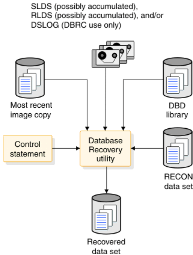
Figure 245. Recovering a database using the IMS Database Recovery utility (DFSURDB0)
