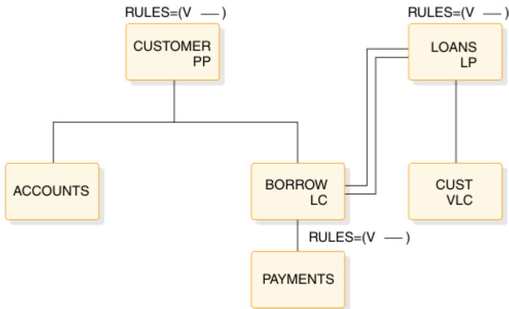
Figure 108. Virtual insert rule example
