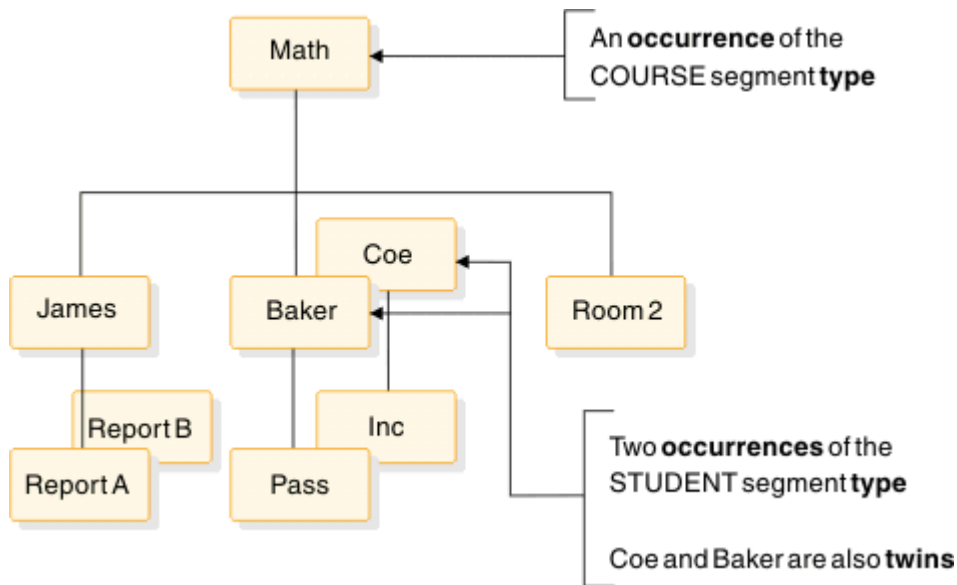
Figure 2. Segment occurrences in a school database record
