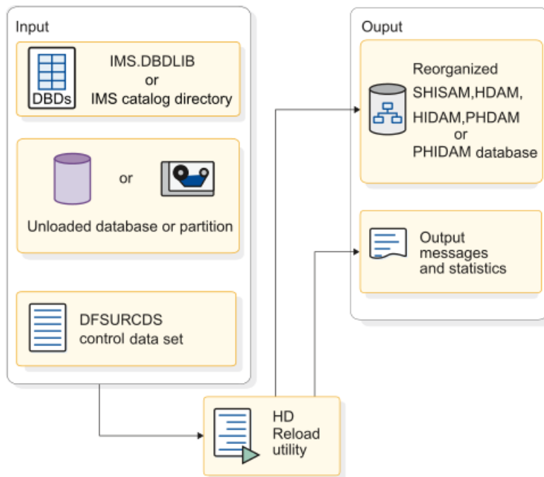
Figure 253. HD Reorganization Reload utility (DFSURGL0)
