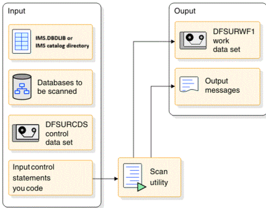
Figure 255. Database Scan utility (DFSURGS0)
