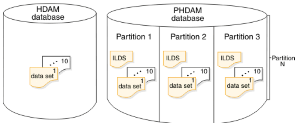
Figure 33. A comparison of the logical views of HDAM and PHDAM databases
