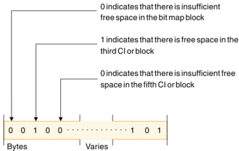
Figure 46. Bitmap for HD databases
