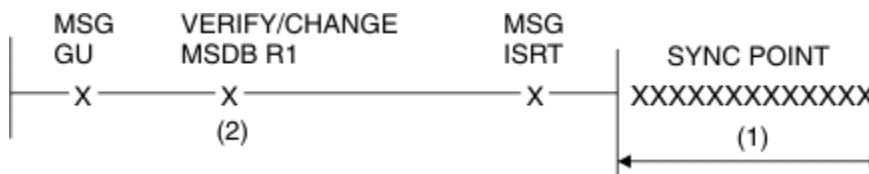
Figure 229. Second example MSDB record held in exclusive mode
