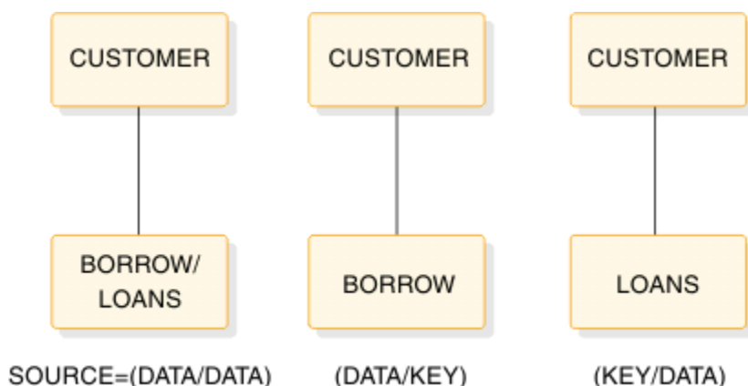
Figure 164. Concatenated segment relationships
