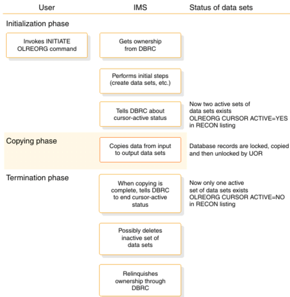
Figure 264. Normal processing steps of HALDB Online Reorganization
