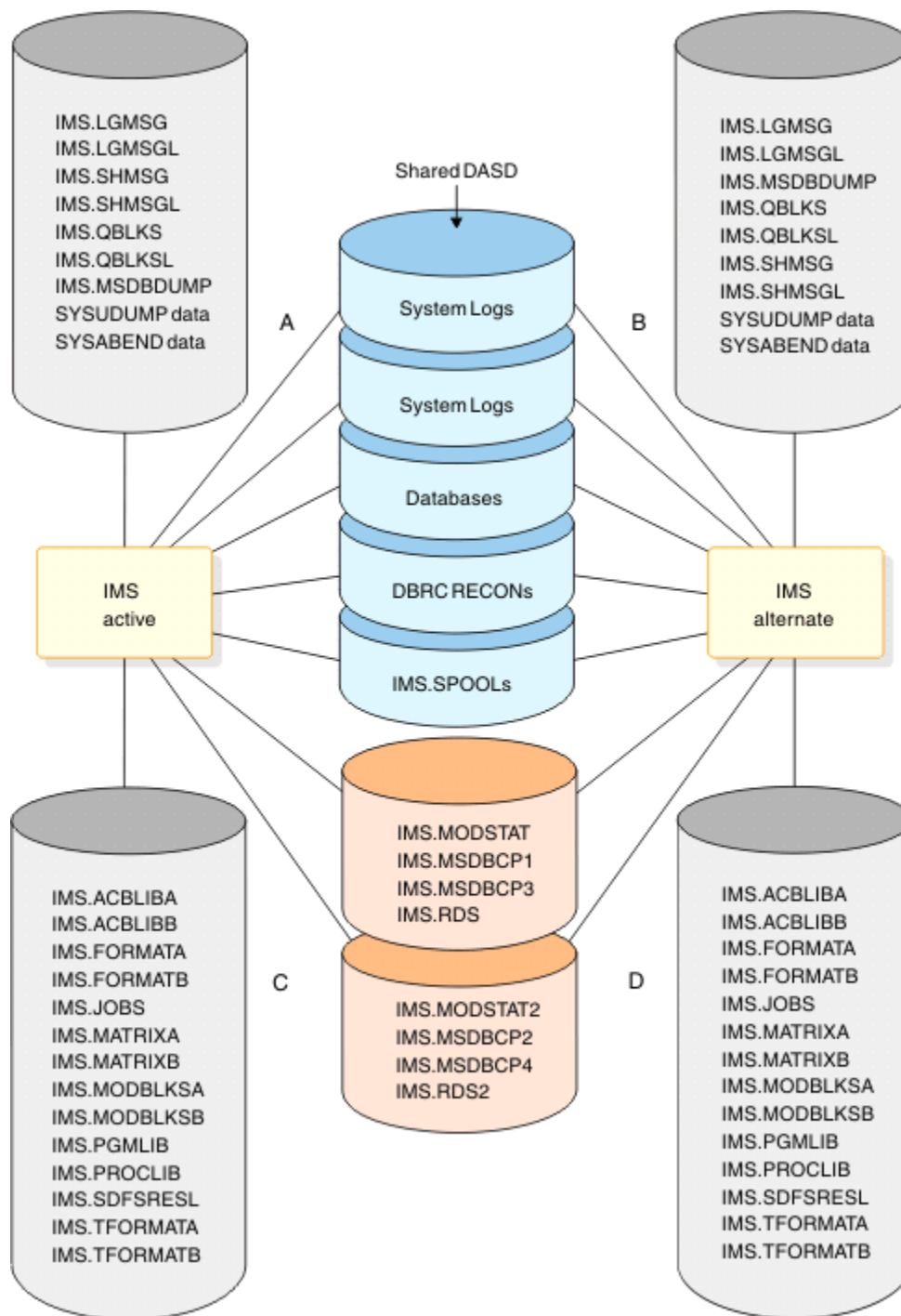
Figure 85. Recommended data set placement
