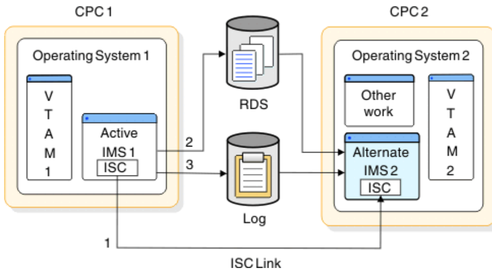
Figure 68. Surveillance options
