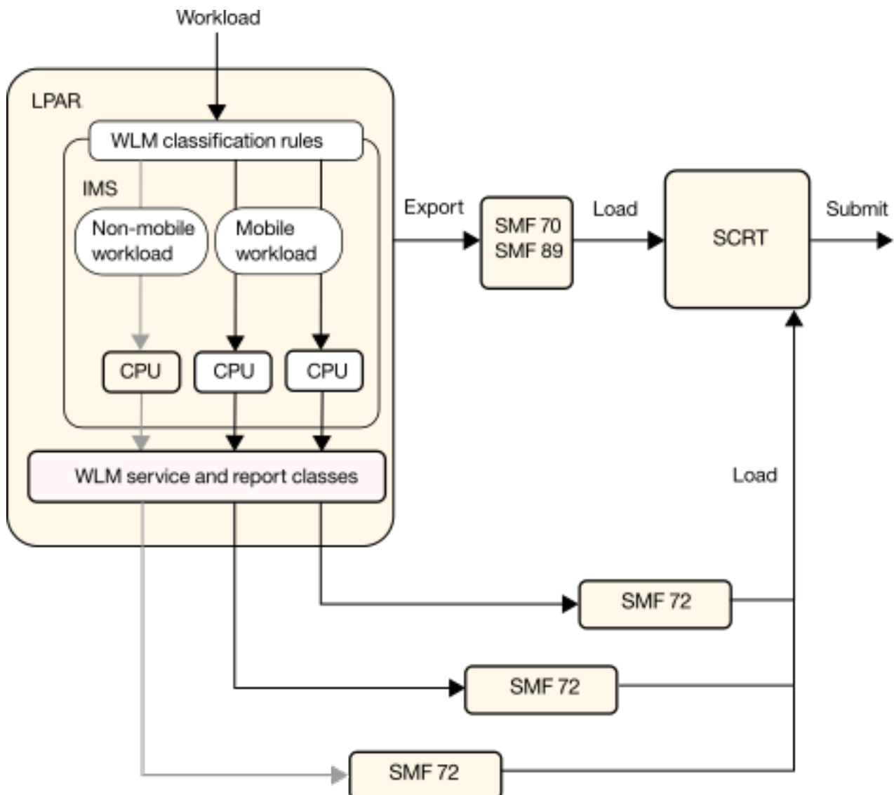
Figure 43. Generating workload reports with WLM classification rules
