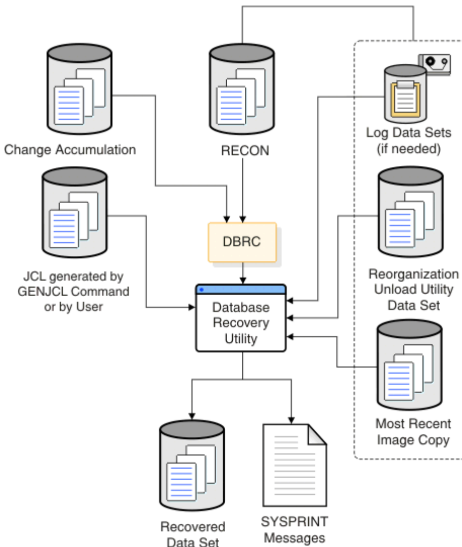
Figure 57. How DBRC works with the Database Recovery utility
