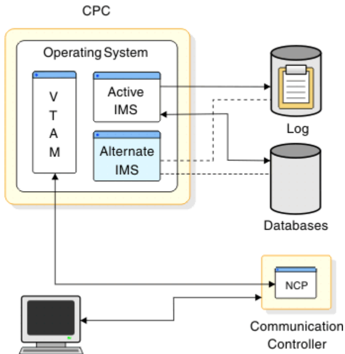
Figure 79. One XRF complex in one CPC
