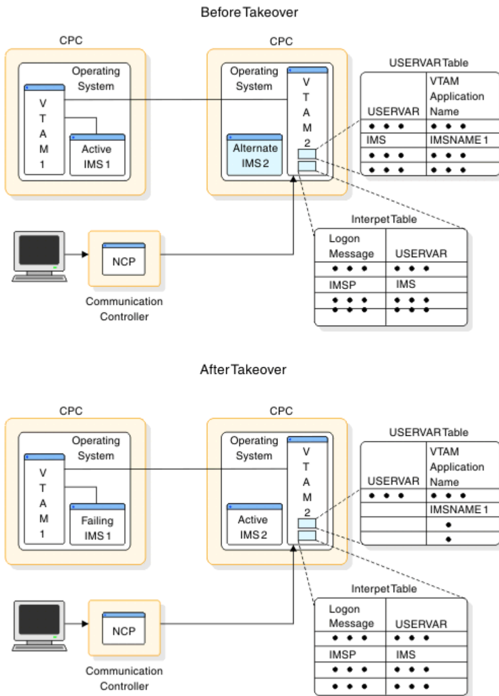
Figure 70. VTAM processing of the logon in an XRF complex that uses USERVAR
