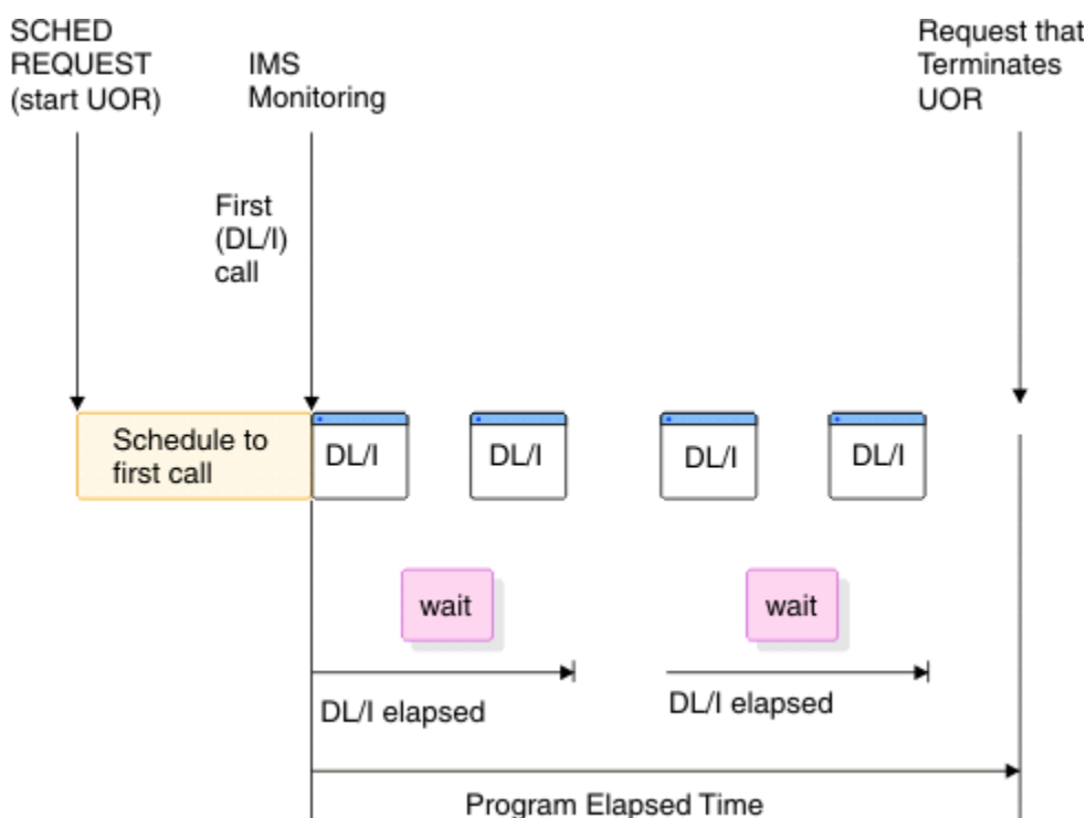
Figure 90. Event intervals
