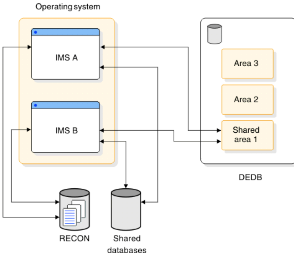
Figure 31. Database-level sharing
