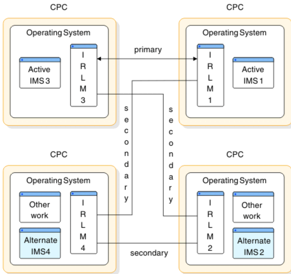
Figure 76. Two data-sharing XRF complexes
