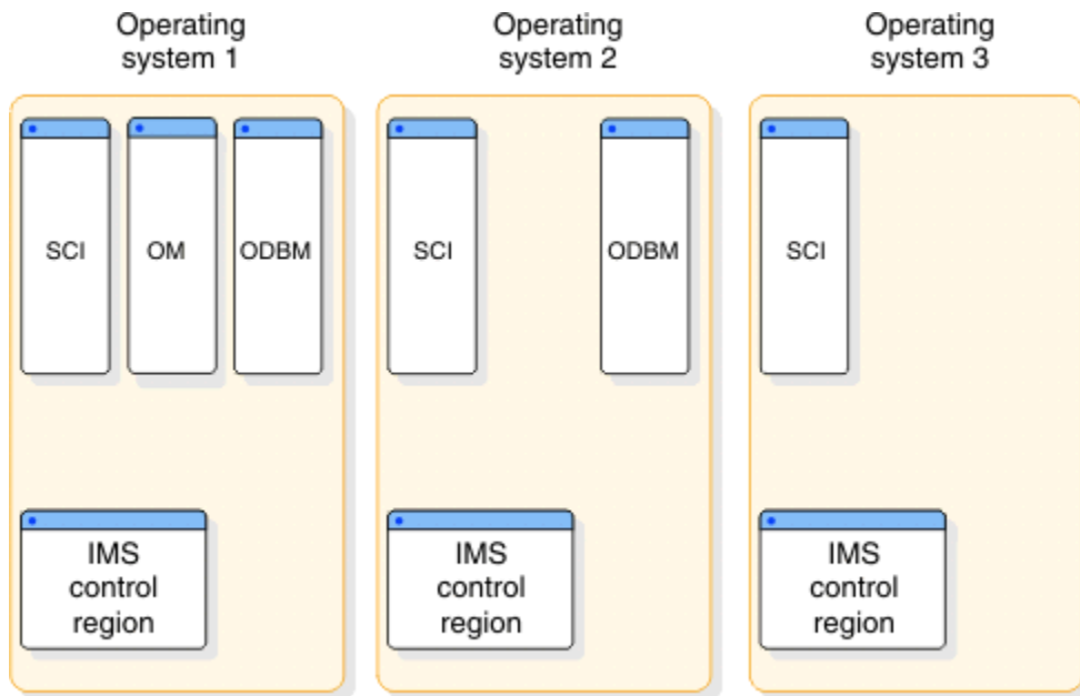
Figure 16. IMSplex minimum ODBM configuration
