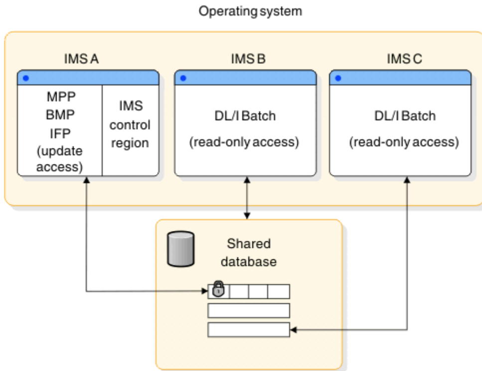
Figure 32. Example of data sharing at the database level with update access
