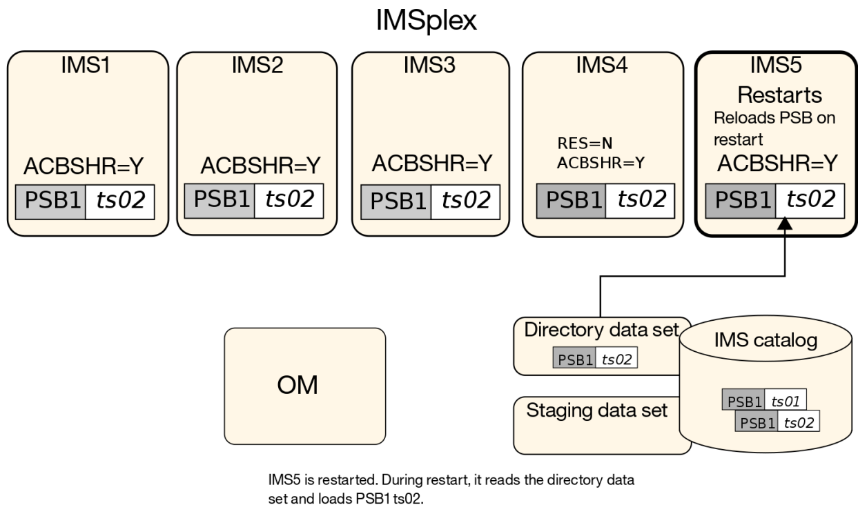
Figure 51. IMS5 restarts and loads the new version of PSB1
