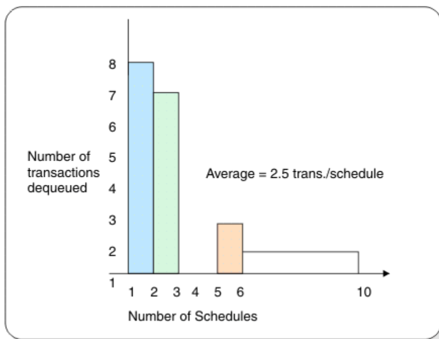
Figure 88. Number of transactions processed for each scheduling of an application program
