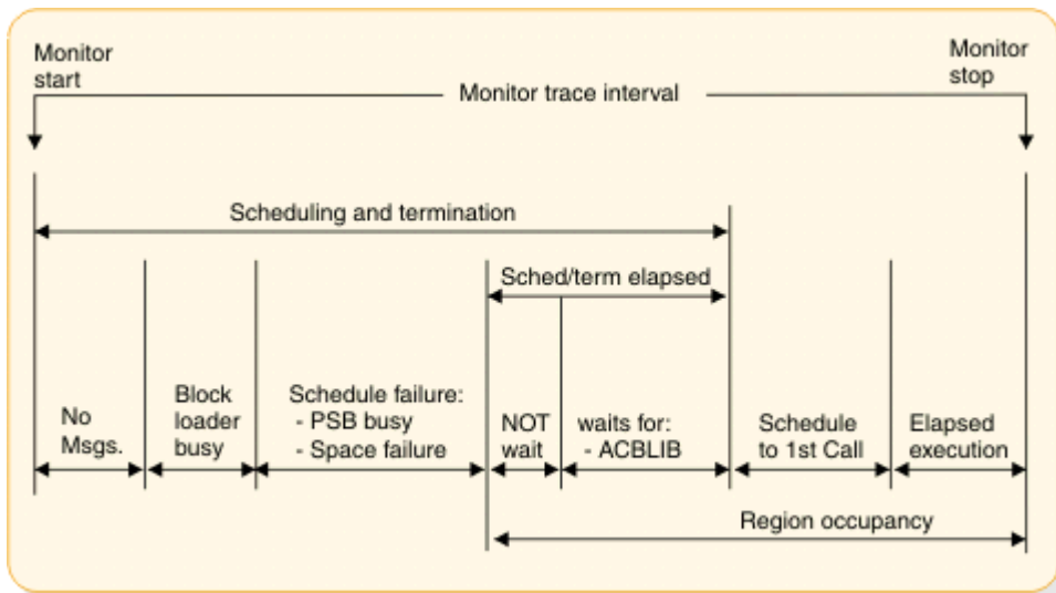
Figure 91. IMS Monitor trace event intervals
