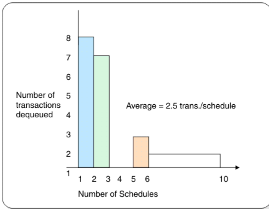
Figure 93. Number of transactions processed for each scheduling of an application program
