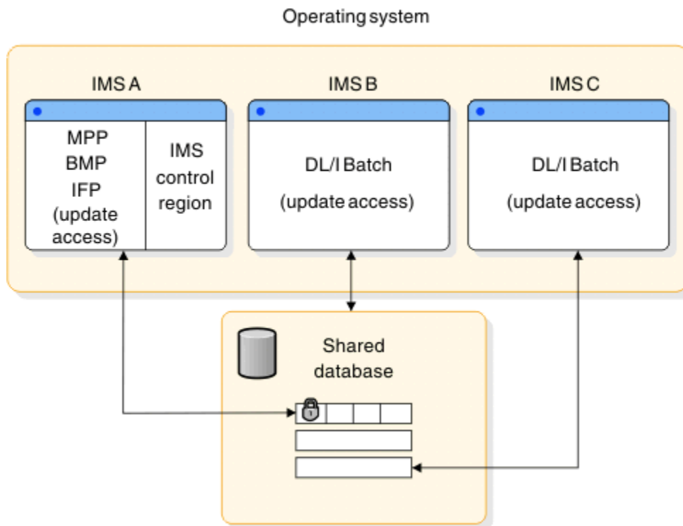
Figure 34. Example of data sharing at the block level with update access
