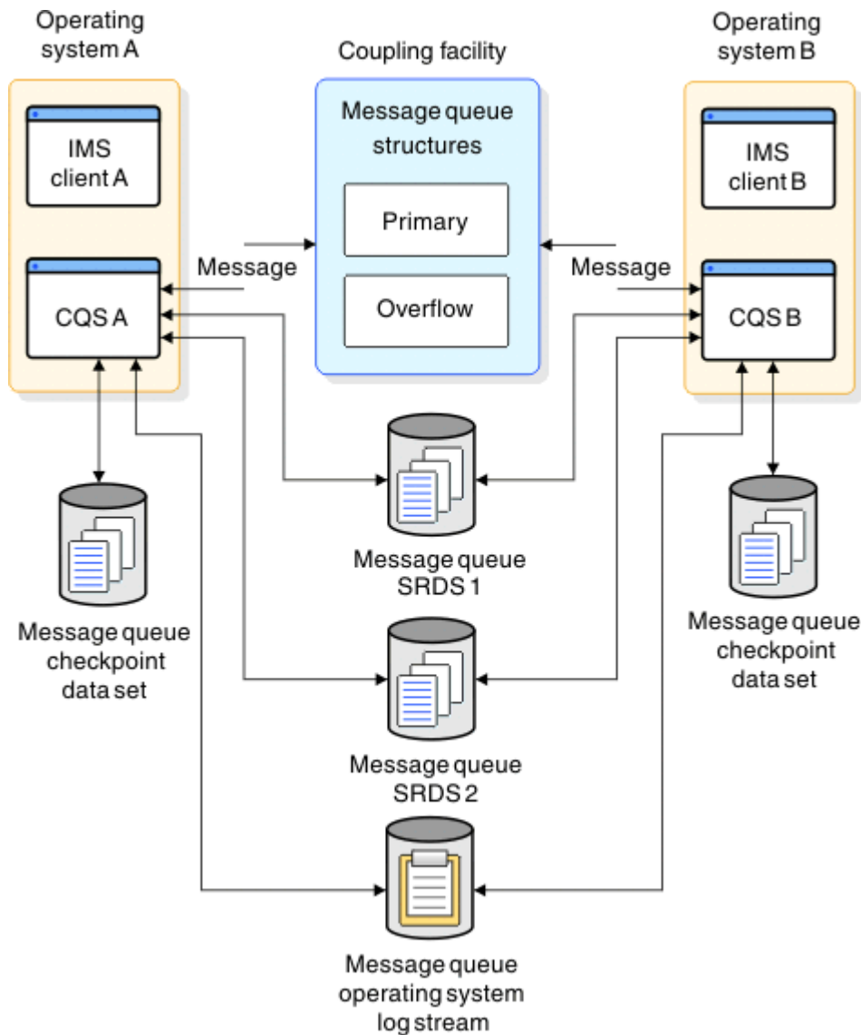
Figure 29. Shared-queues environment with its message queue (MSGQ) list structures
