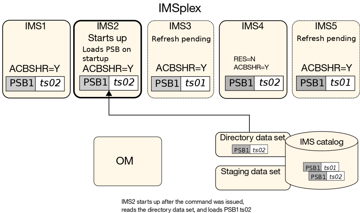
Figure 49. IMS2 loads PSB1 during restart
