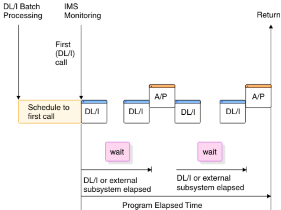
Figure 92. Elapsed Time event intervals
