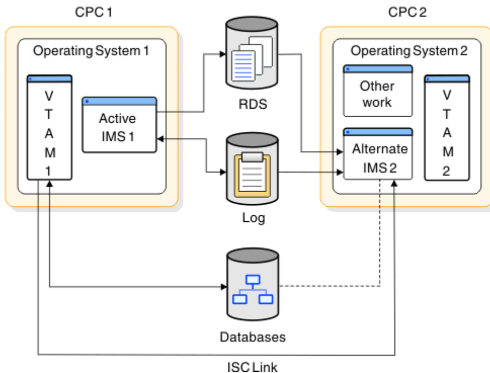
Figure 65. The XRF complex before a takeover
