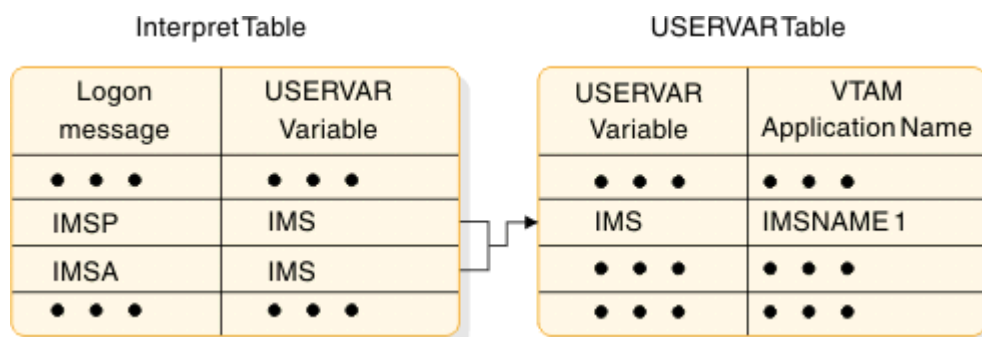
Figure 69. The interpret and USERVAR tables
