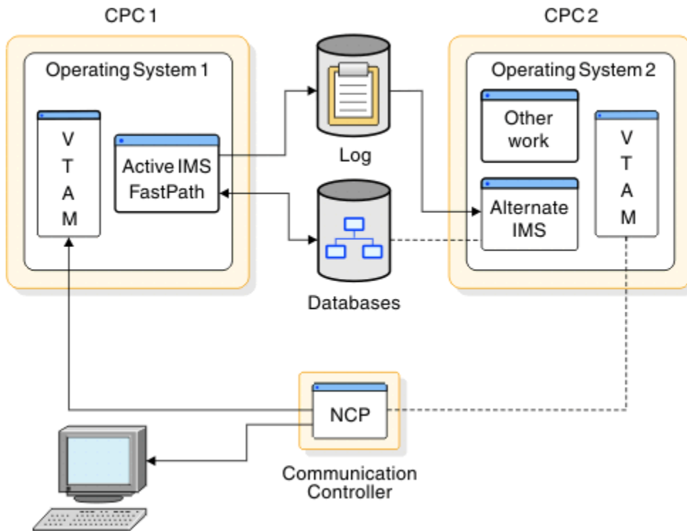
Figure 80. One XRF complex in two CPCs
