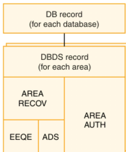
Figure 64. DBRC Fast Path database records
