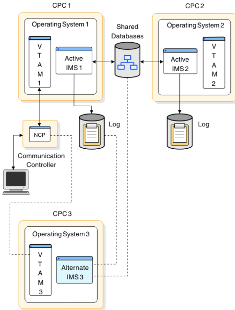
Figure 81. One XRF complex in two CPCs and a non-XRF IMS
