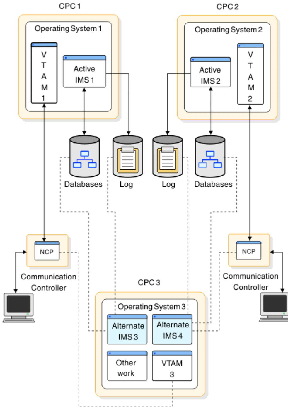
Figure 82. Two XRF complexes in three CPCs
