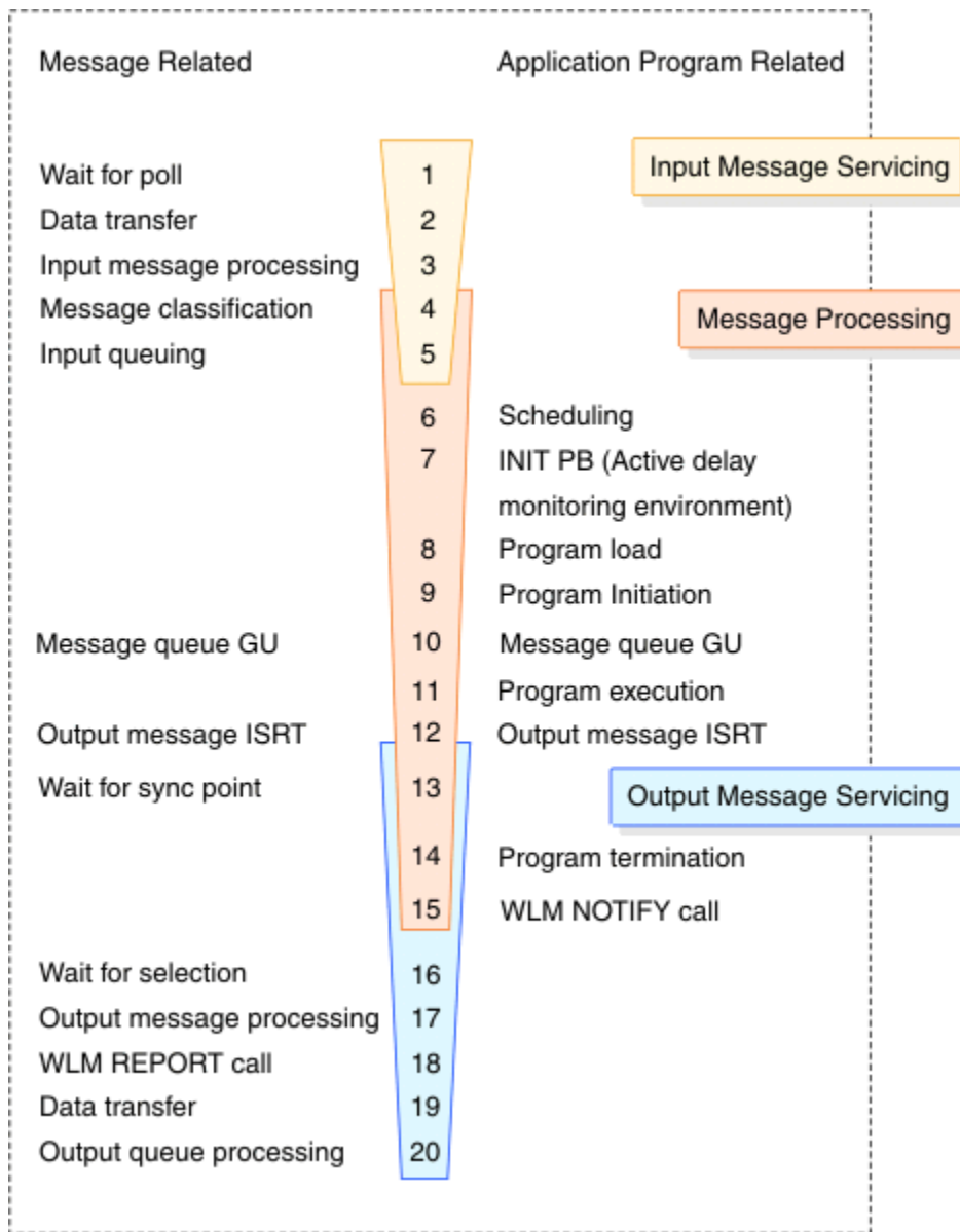
Figure 44. Processing events during transaction flow through IMS
