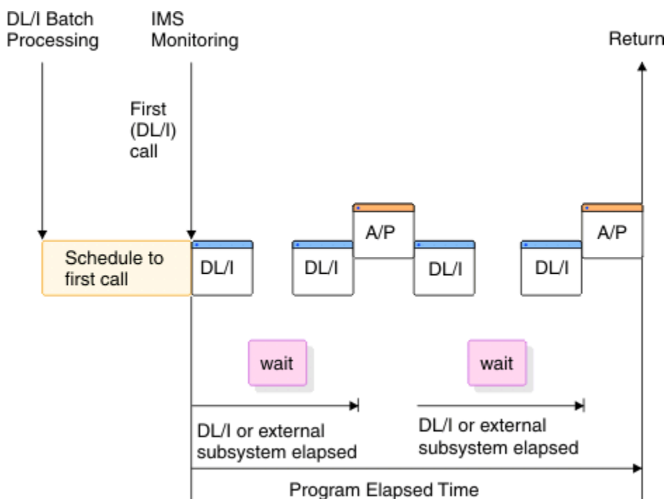
Figure 87. Event intervals for time in application code and DL/I processing
