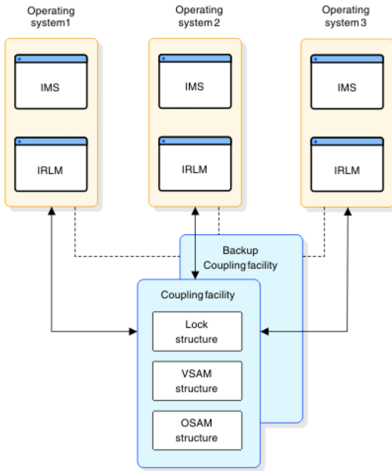
Figure 38. Sysplex data-sharing configuration with three structures on one coupling facility with backup
