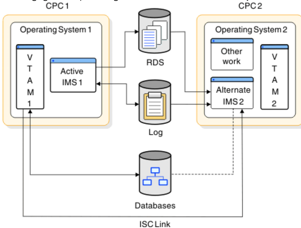
Figure 74. XRF synchronization phase
