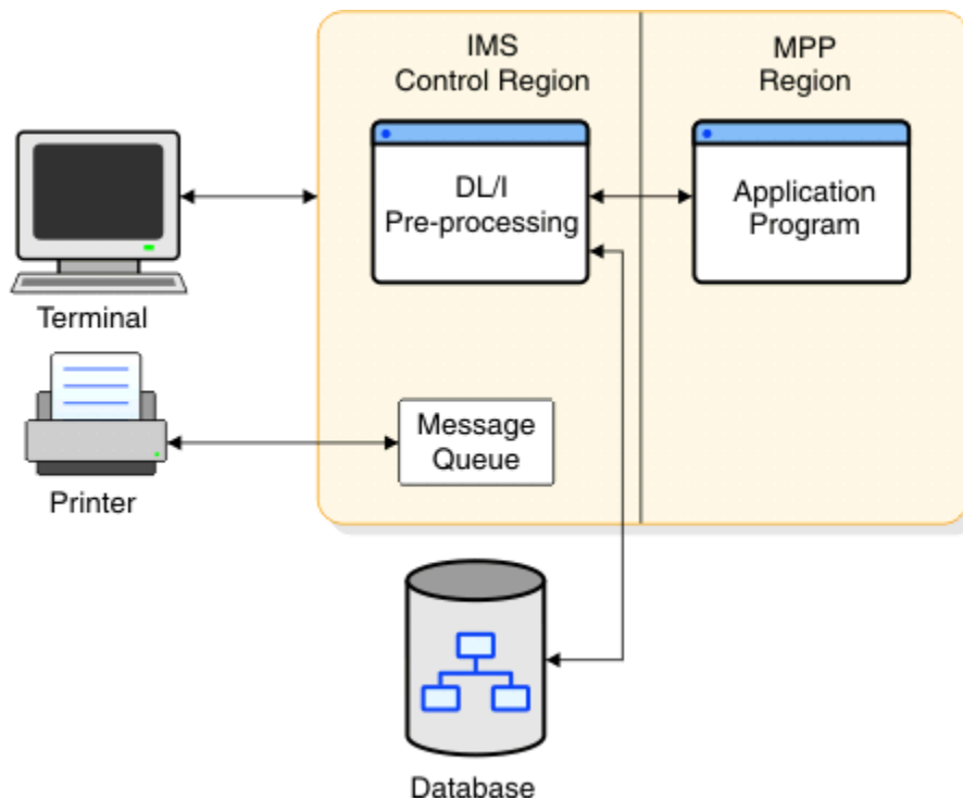
Figure 53. IMS environment without Spool API
