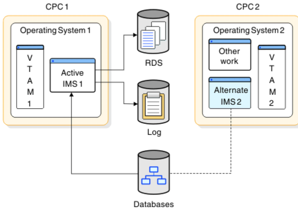
Figure 73. XRF initialization phase
