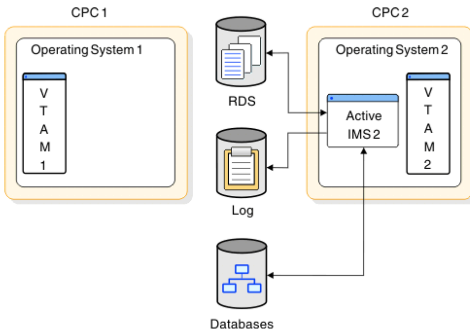
Figure 78. XRF termination phase
