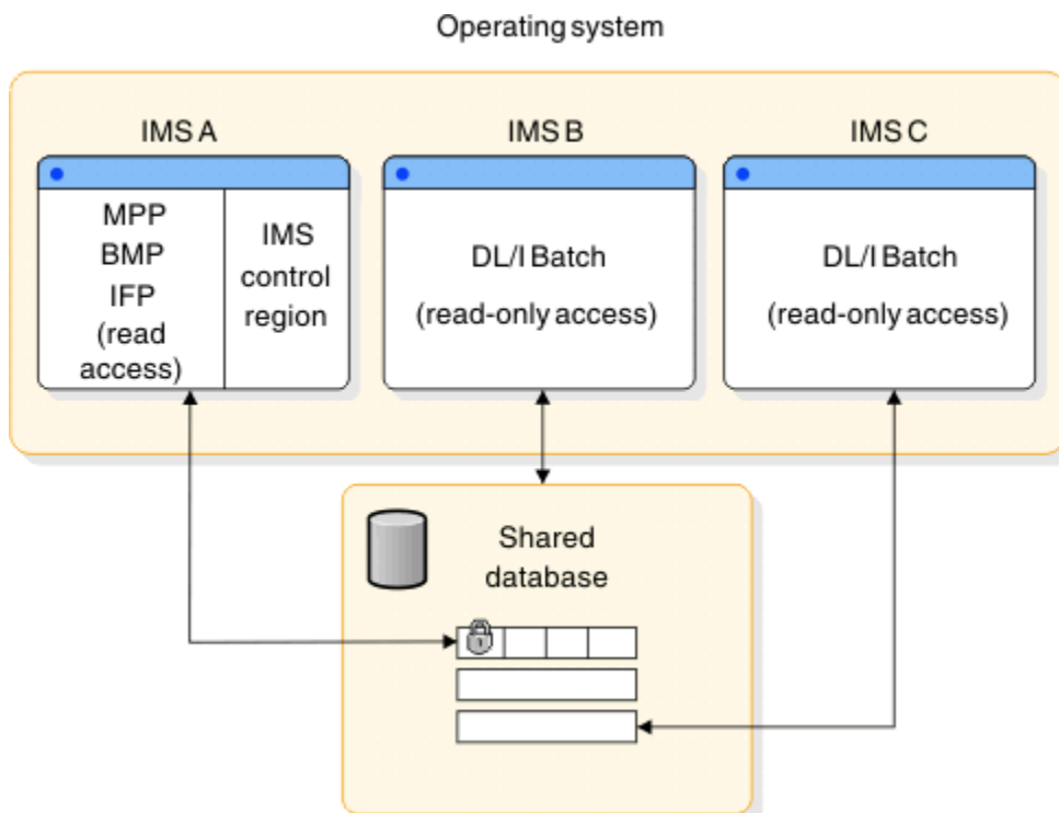
Figure 33. Example of data sharing at the database level with read access
