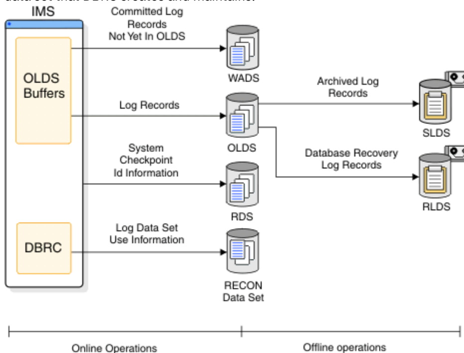
Figure 55. Logs produced for recovery and restart
