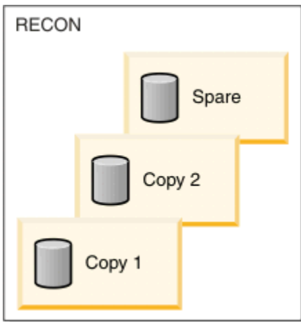
Figure 60. DBRC dual RECON set up with a spare
