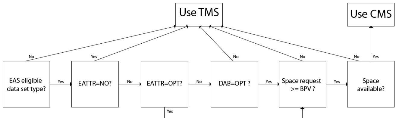
Figure 8. EAV Logic
