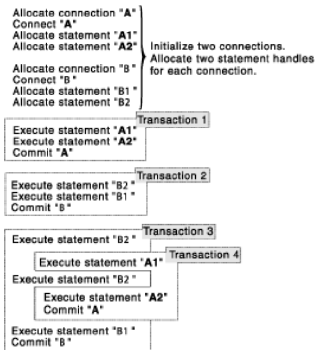
Figure 39. Multiple connections with concurrent transactions
