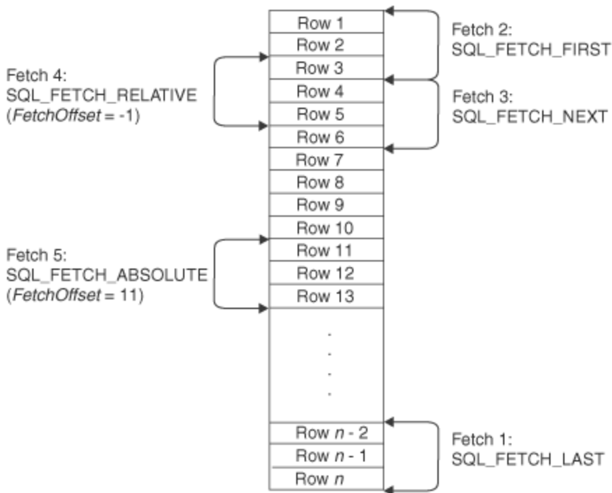
Figure 50. Example of cursor movement after SQLFetchScroll() calls
