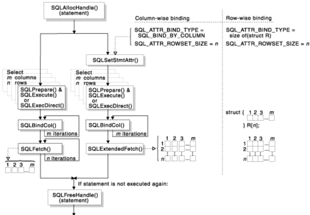
Figure 48. Array retrieval
