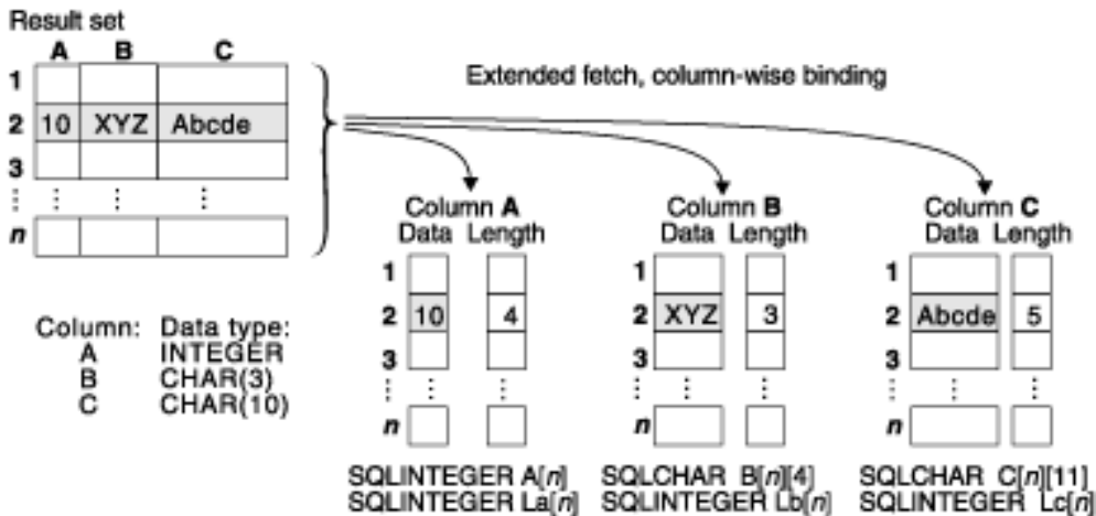
Figure 46. Column-wise binding
