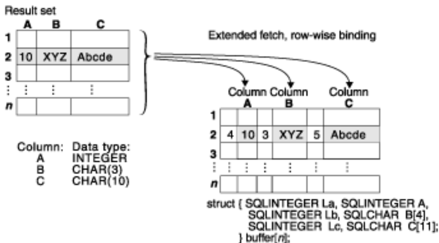
Figure 47. Row-wise binding
