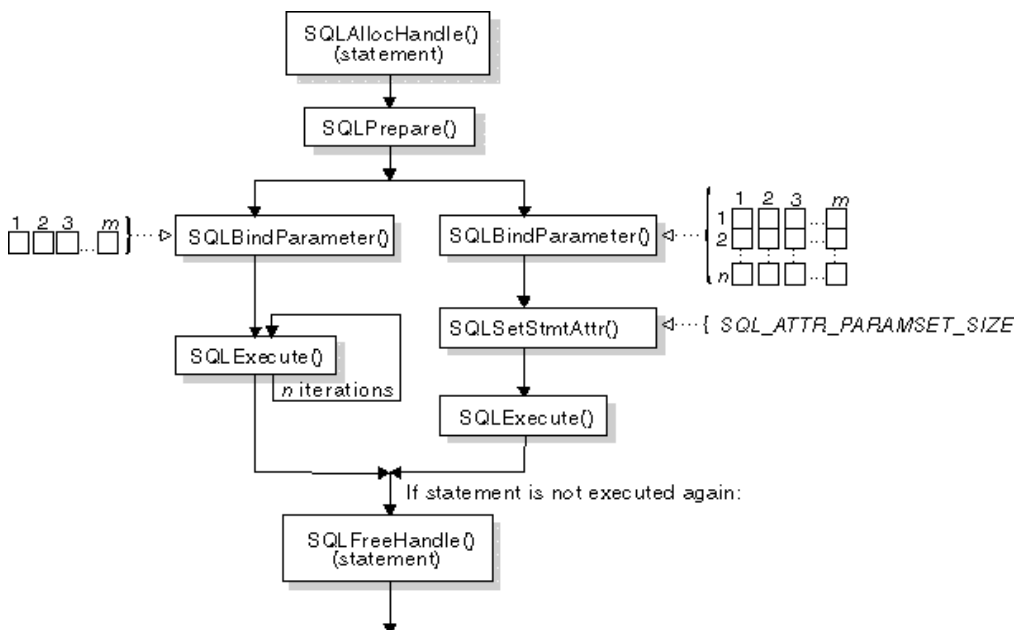
Figure 43. Array insert
