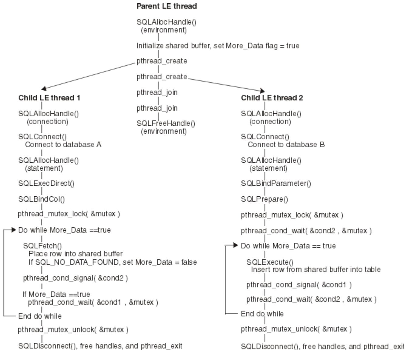
Figure 61. Multithreaded application
