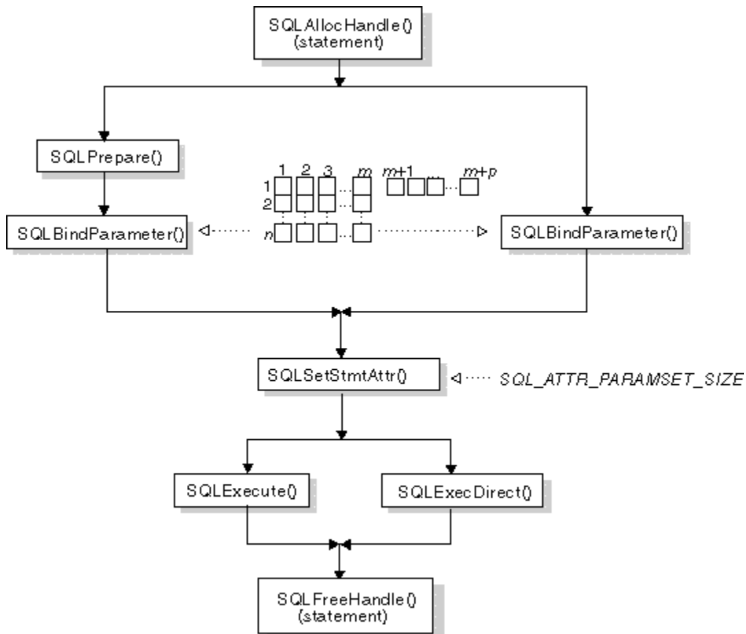
Figure 44. Array merge
