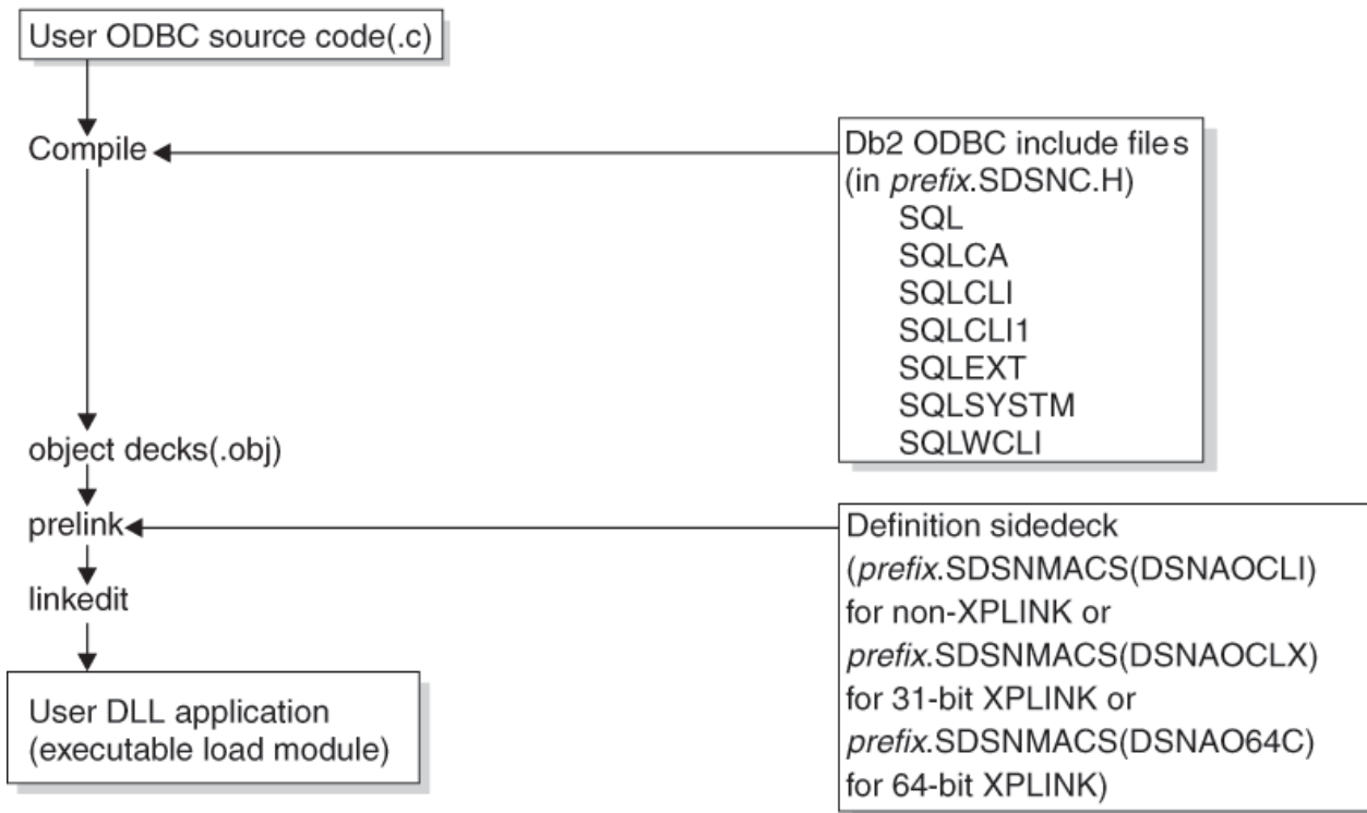
Figure 8. Db2 ODBC program preparation
