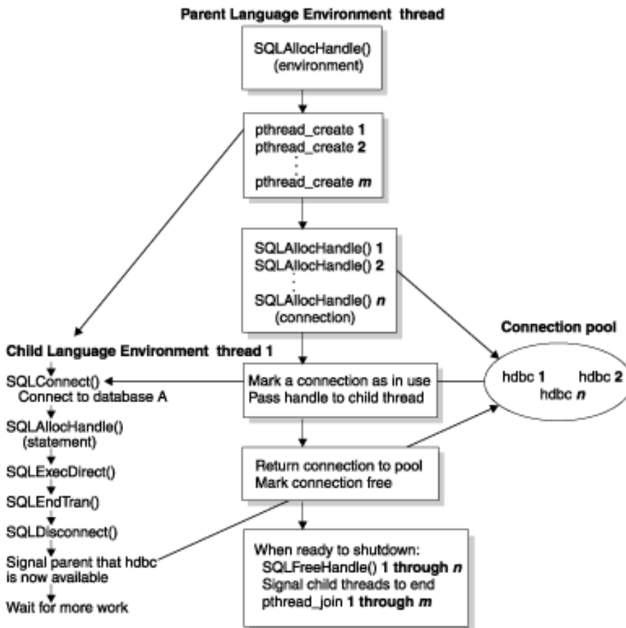
Figure 64. Model for multithreading with connection pooling (MULTICONTEXT=1)
