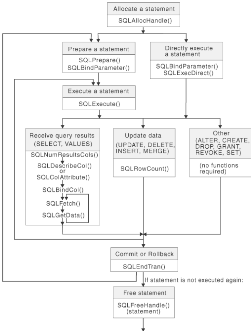
Figure 4. Transaction processing
