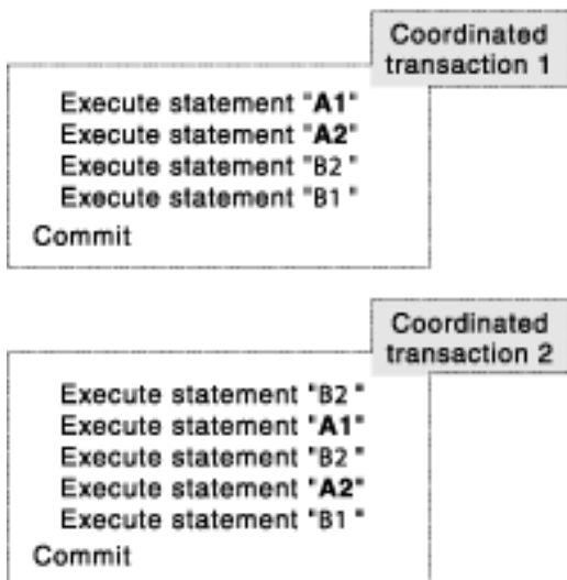
Figure 40. Multiple connections with coordinated transactions
