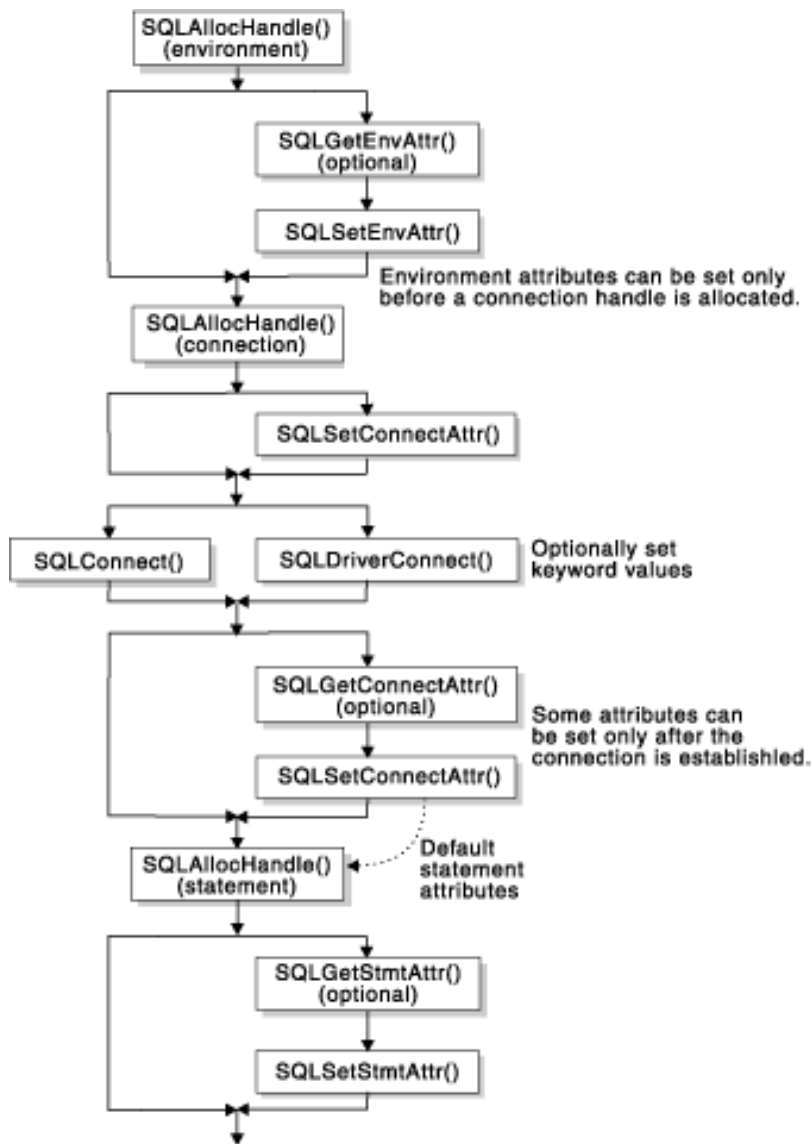
Figure 37. Setting and retrieving attributes
