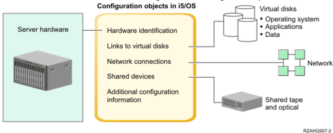
Figure 1. Integrated server overview
