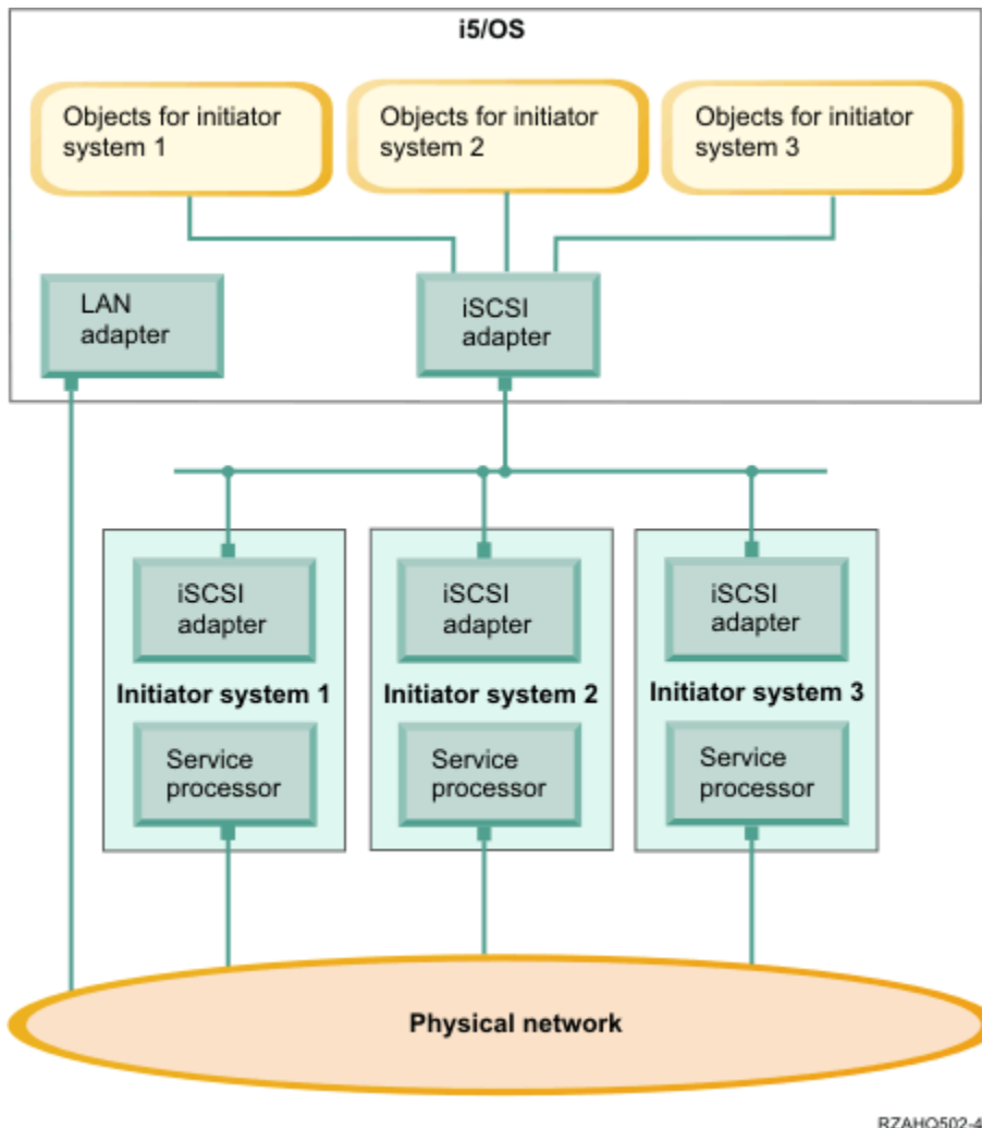
Figure 5. Multiple iSCSI-attached servers
