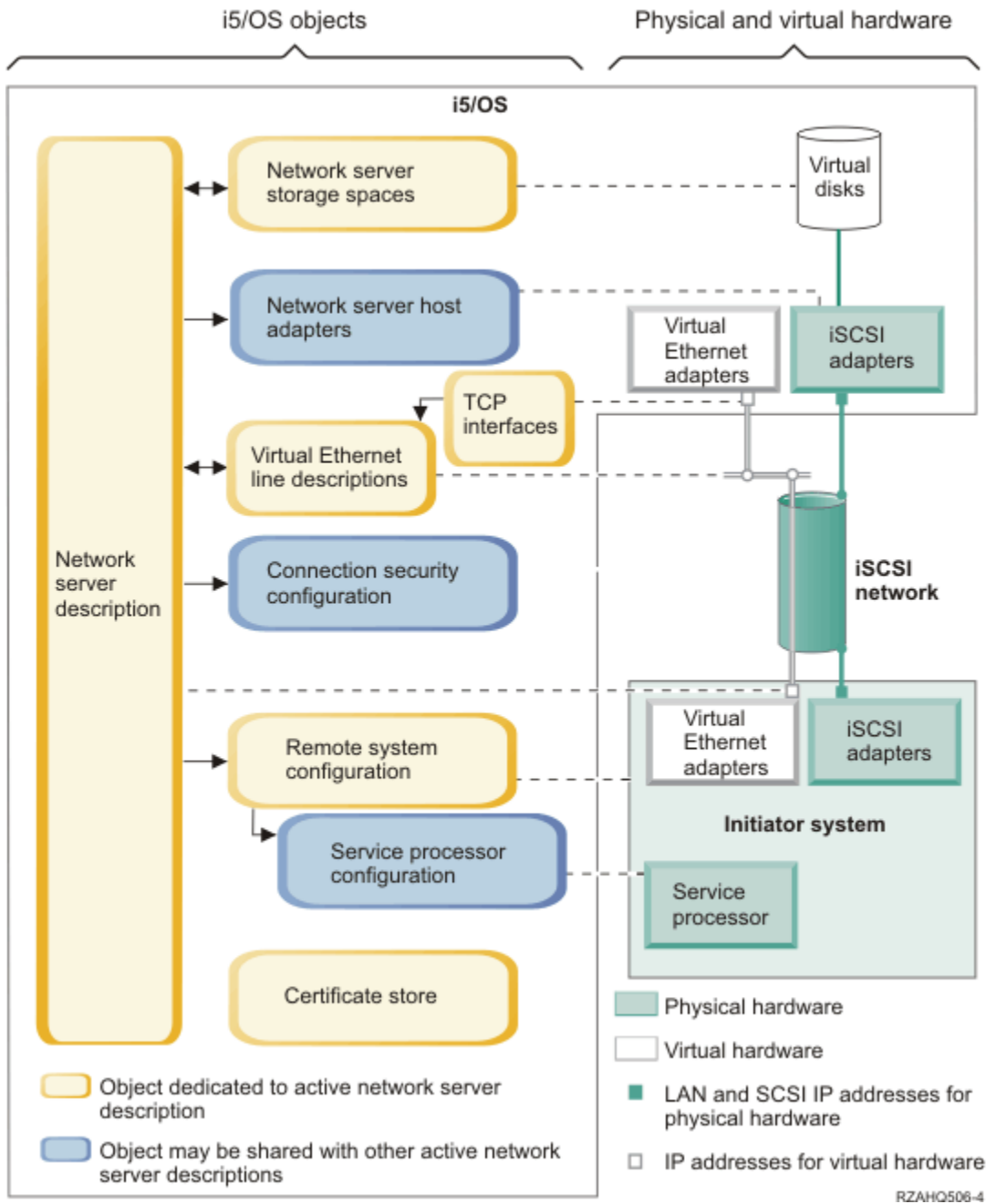
Figure 10. iSCSI configuration objects in IBM i
