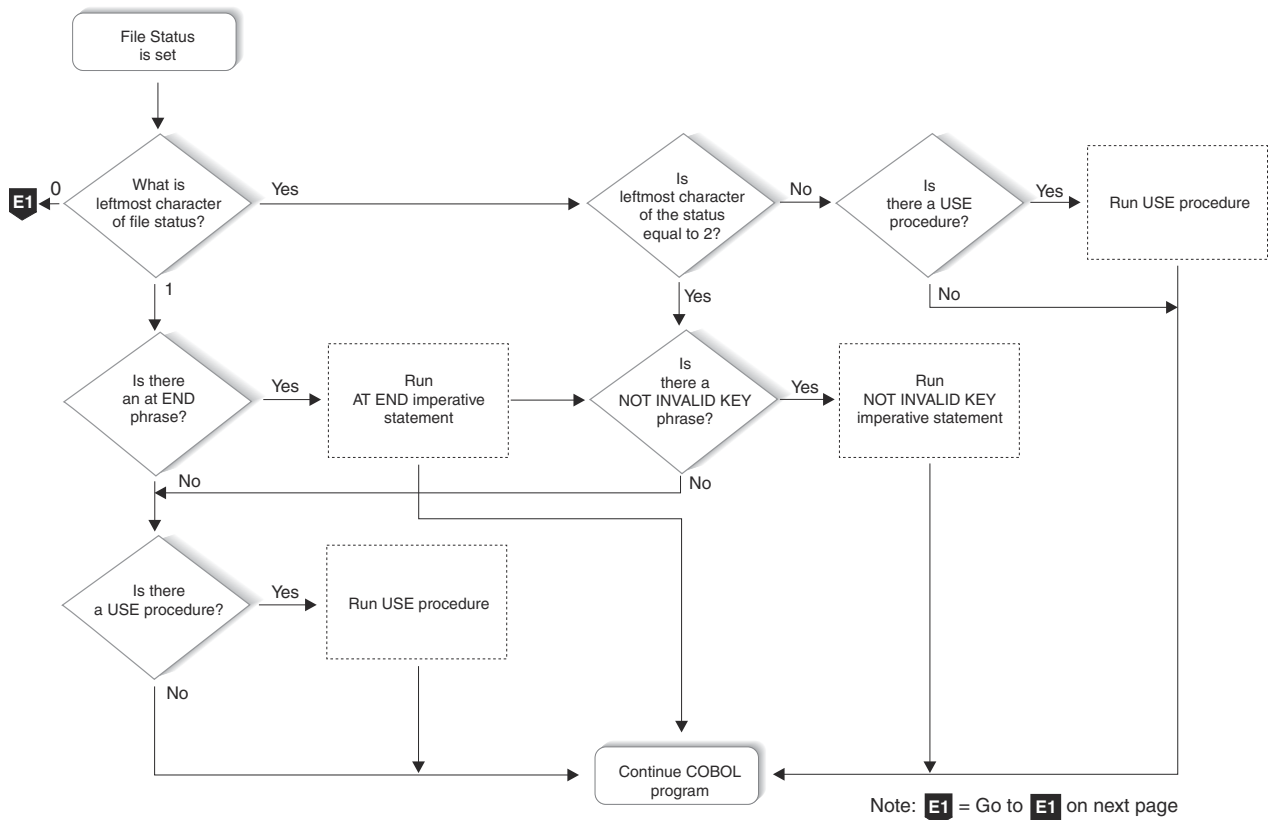
Figure 88. Processing of I/O Verbs
