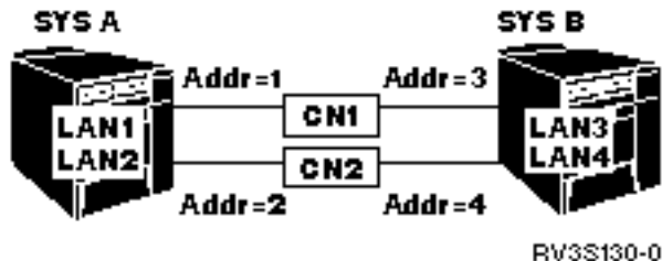
Figure 3. Correct configuration showing two connection networks and two LAN lines
