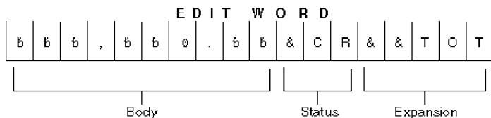
Figure 112. Parts of an Edit Word
