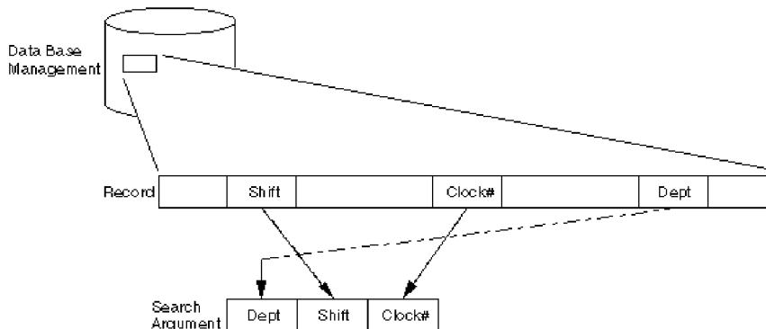
Figure 335. KLIST and KFLD Operations
