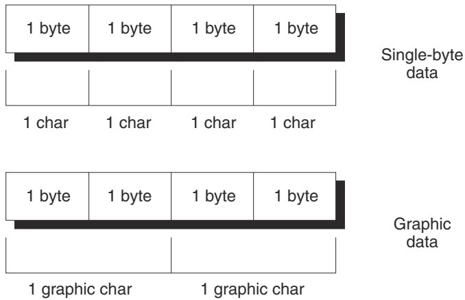
Figure 90. Comparing Single-byte and graphic data
