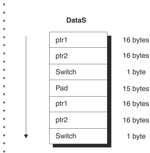
Figure 108. Defining pointers
