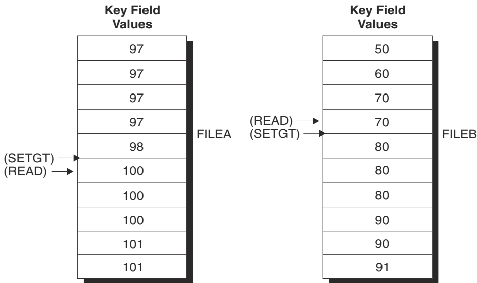
Figure 382. SETGT Operation
