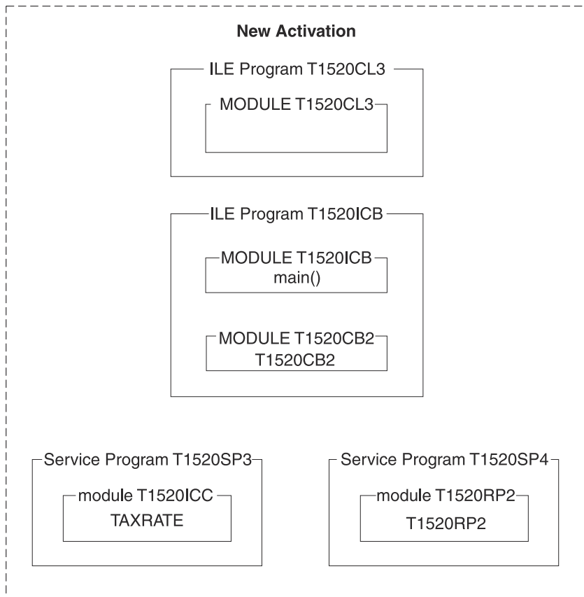
Figure 240. Integrated Language Environment Structure
