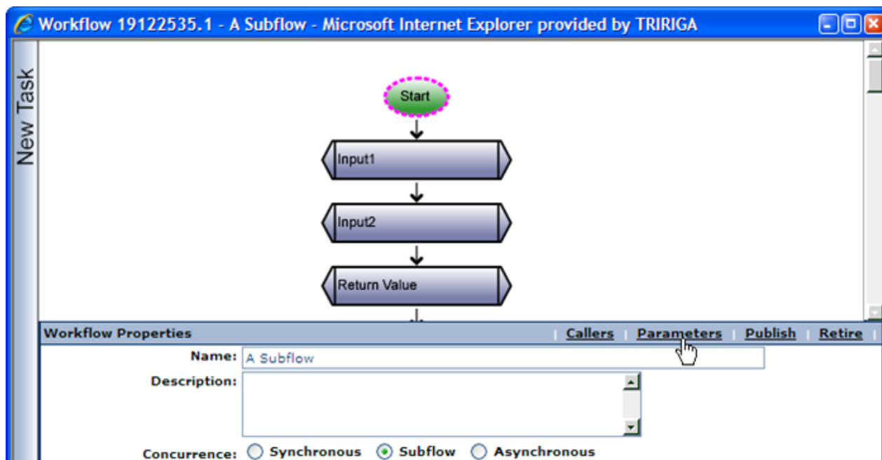
Figure 52. Start task example
