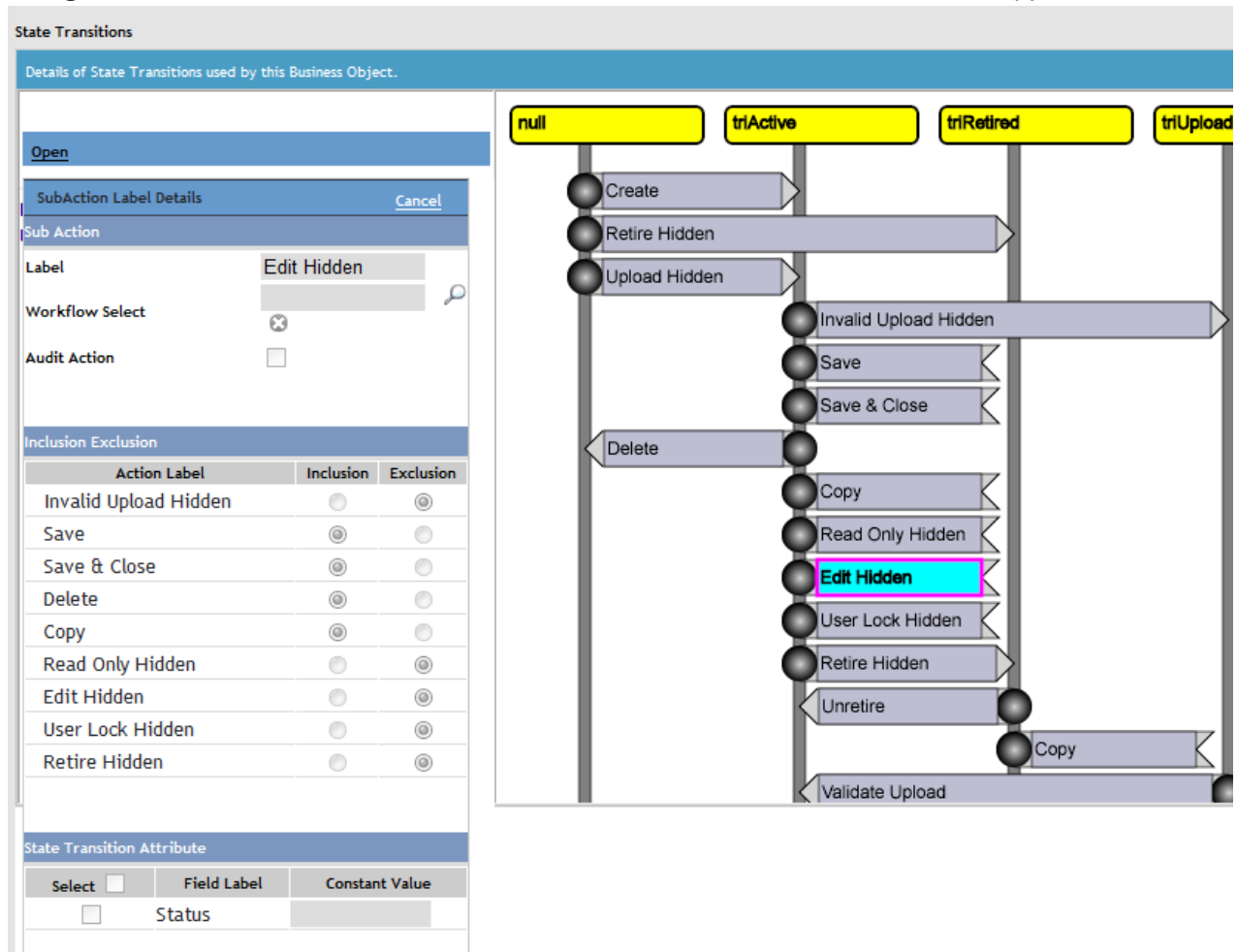
Figure 26. State Transitions panel for hidden sub action
