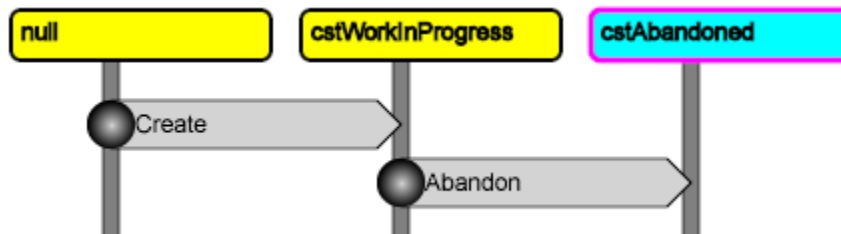
Figure 24. Life cycle diagram with abandoned state added
