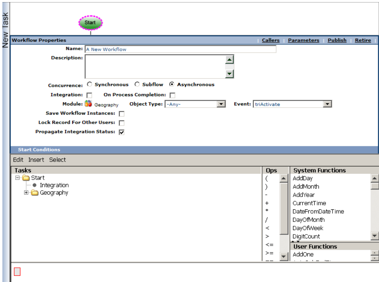
Figure 51. Start Task properties for asynchronous workflow
