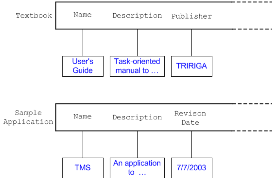
Figure 15. Records that are not links
