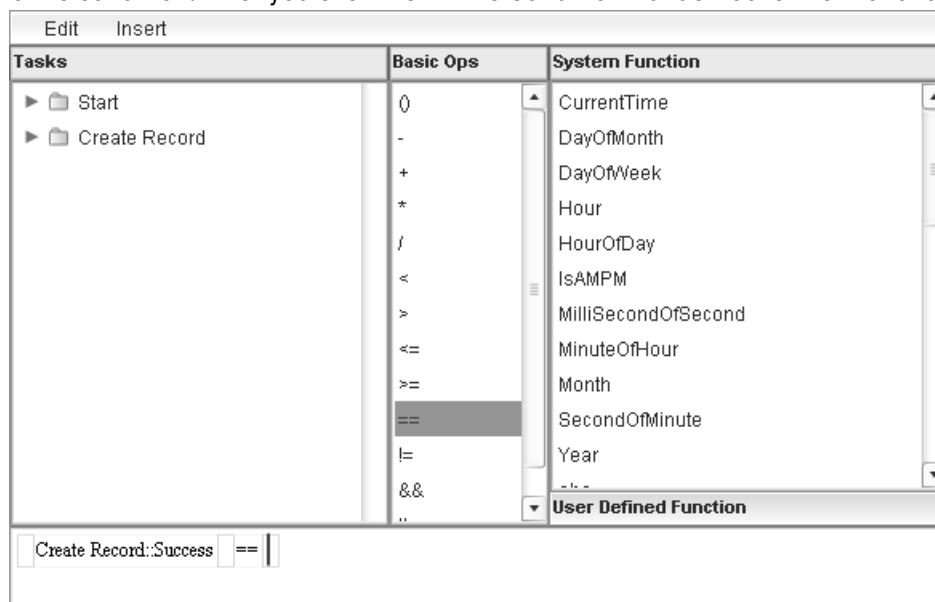
Figure 75. Condition Builder ==
