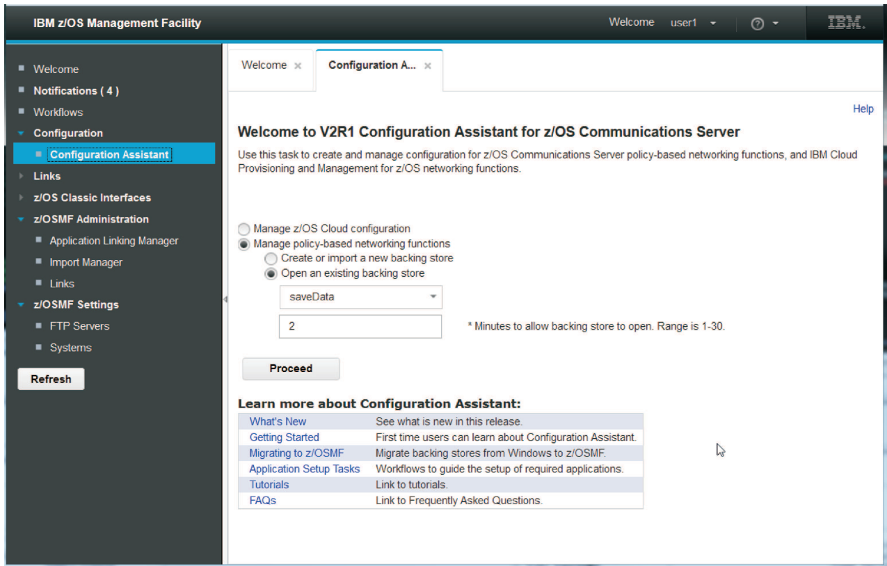
Figure 11. Configuration Assistant task main page
