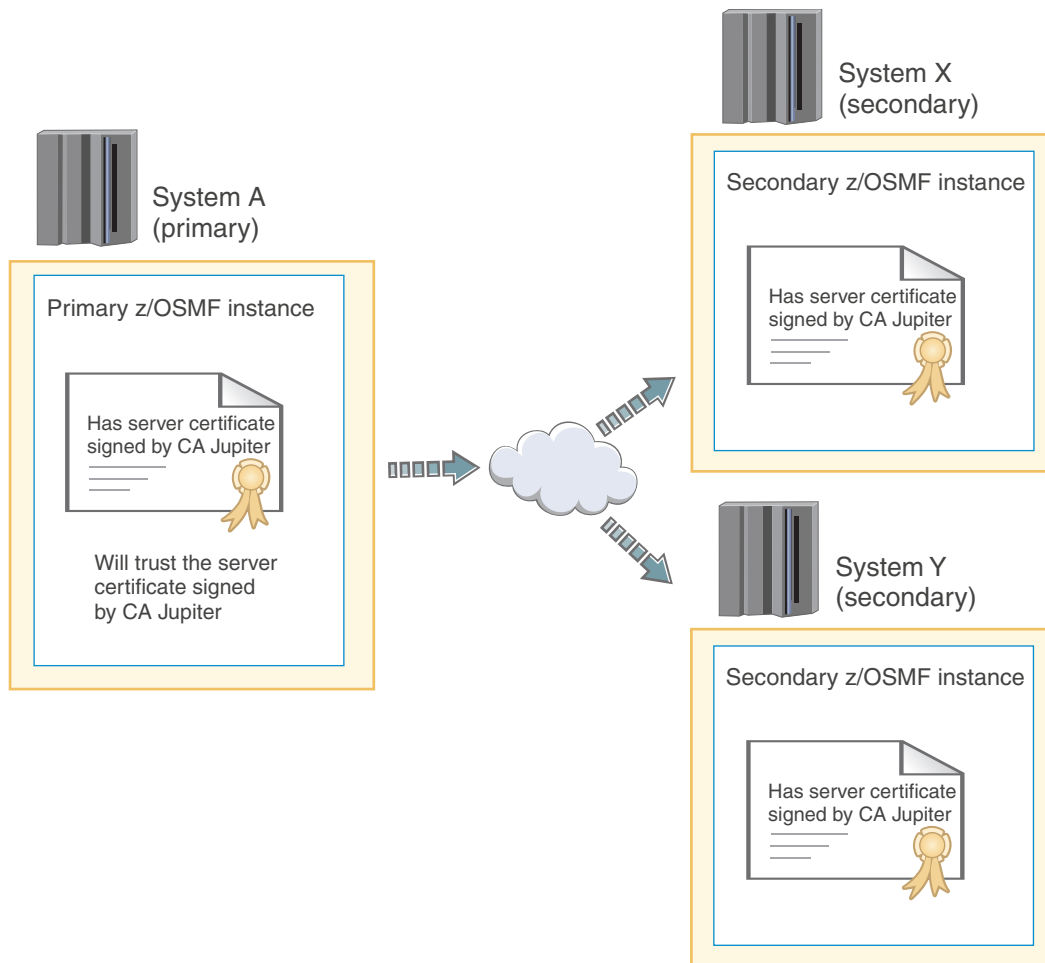
Figure 29. Trust relationship when server certificates are signed by the same CA certificate
