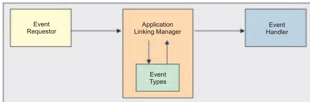
Figure 34. Key components in the application linking process
