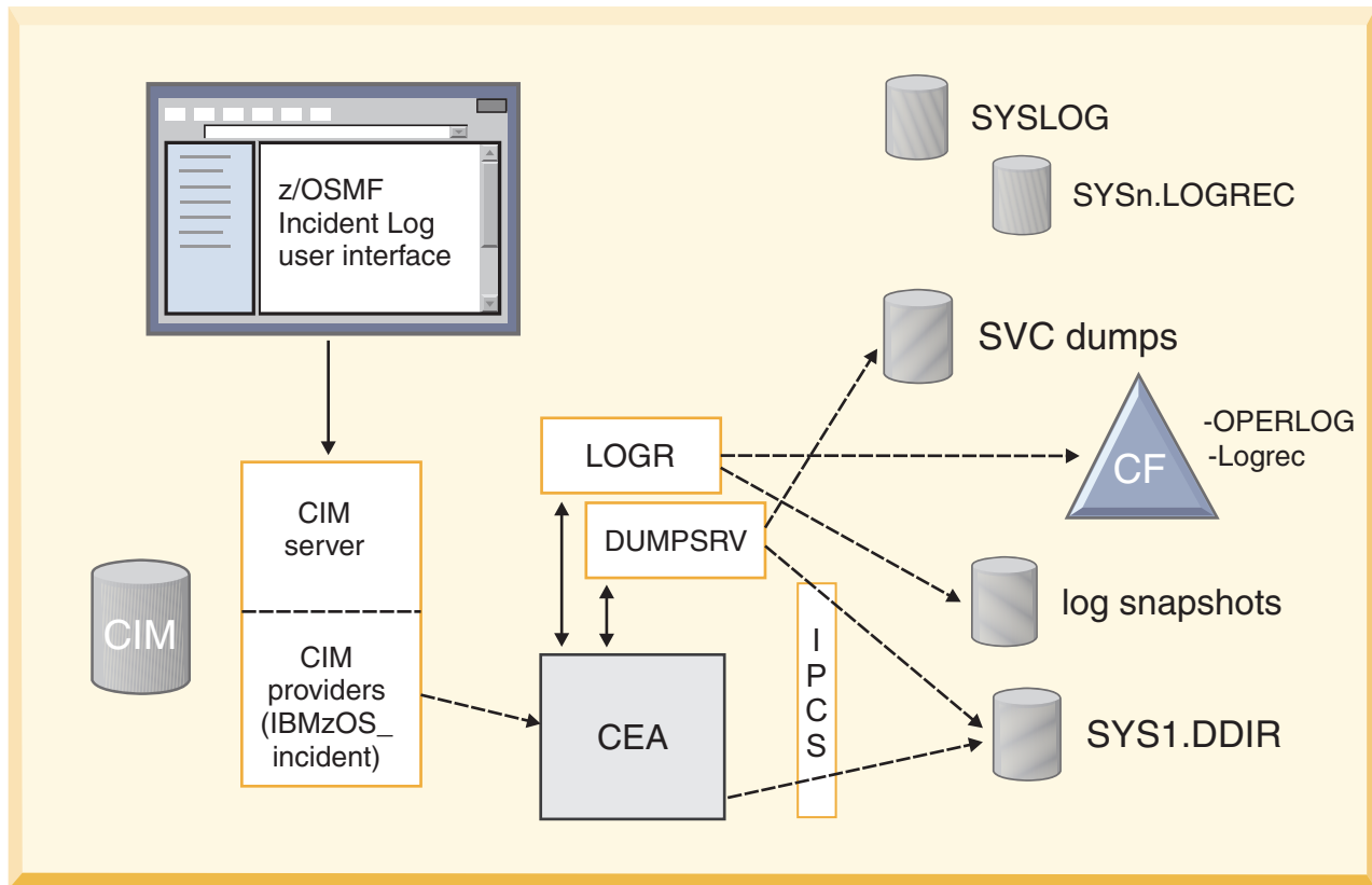
Figure 46. z/OS components that are used in Incident Log task processing
