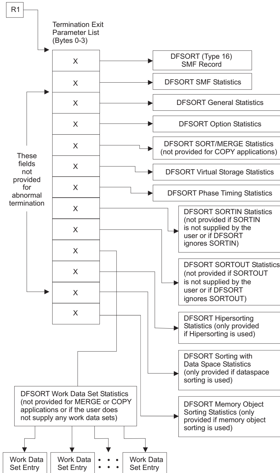
Figure 30. Information DFSORT Passes to Your ICETEXIT
