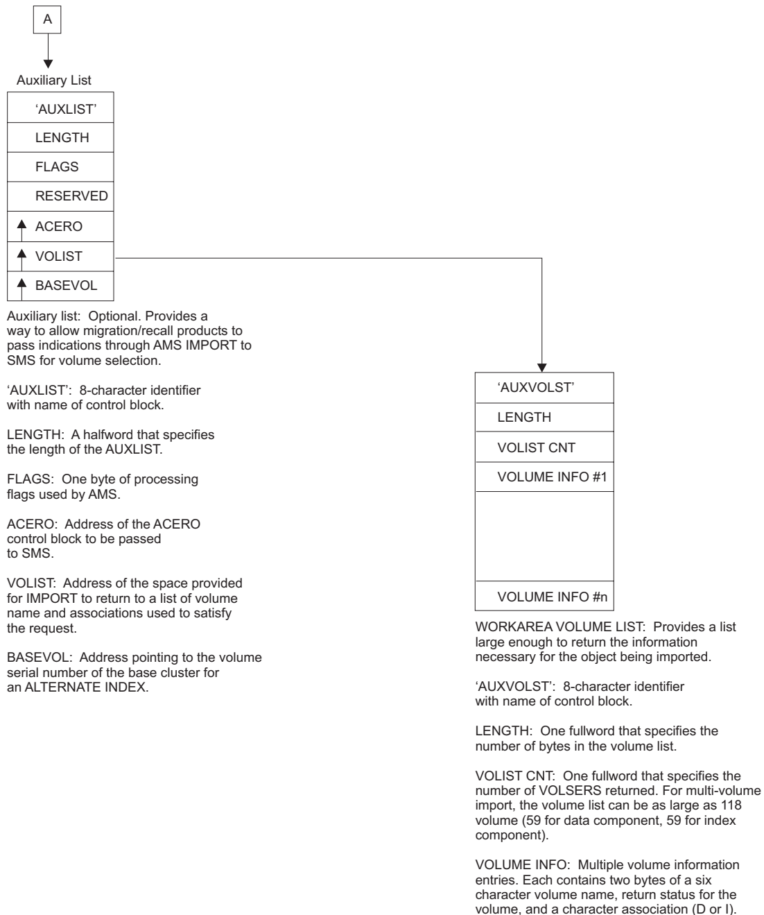
Figure 53. Processor Invocation Argument List from Your Program
