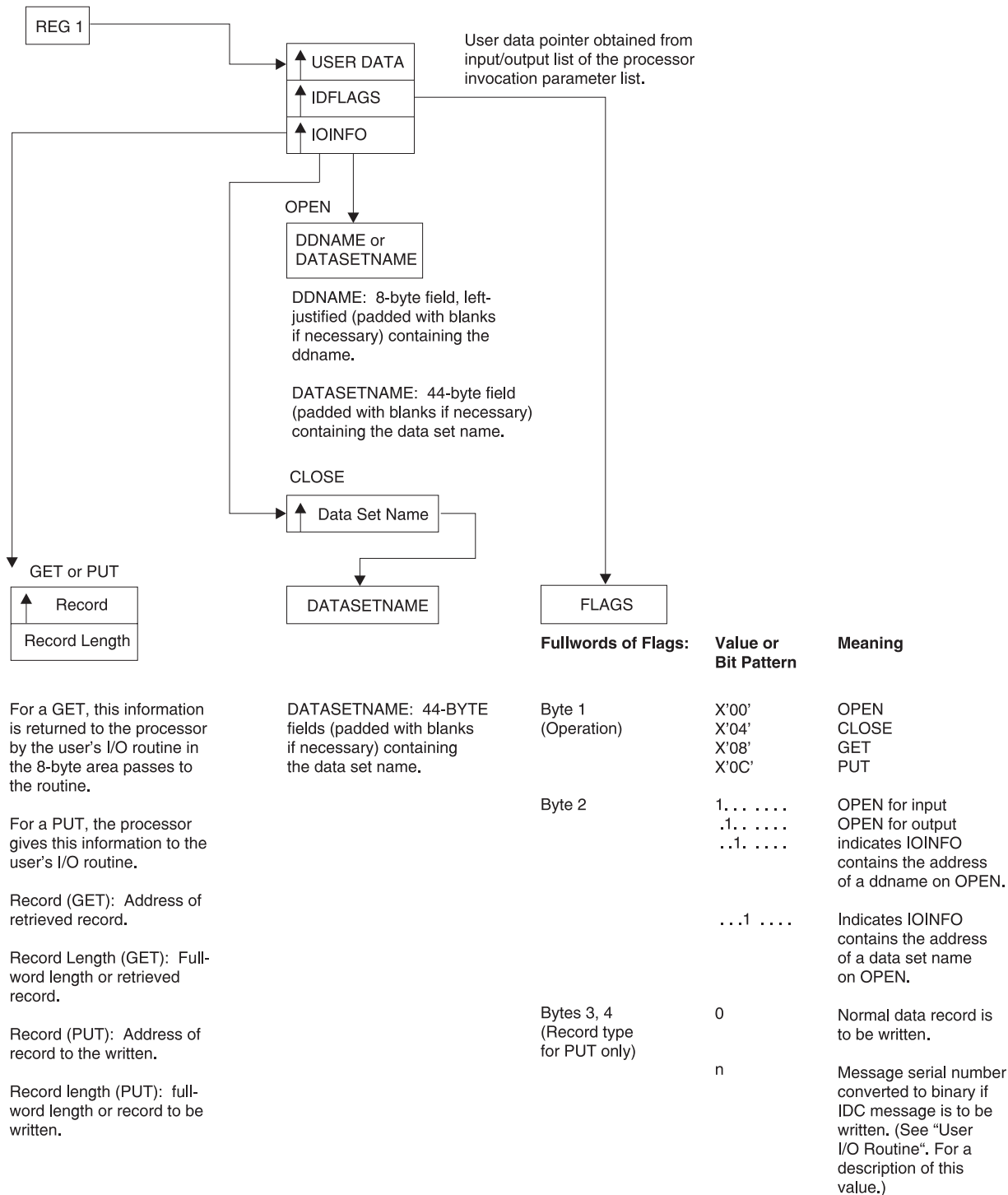
Figure 54. Arguments Passed to and from a User I/O Routine
