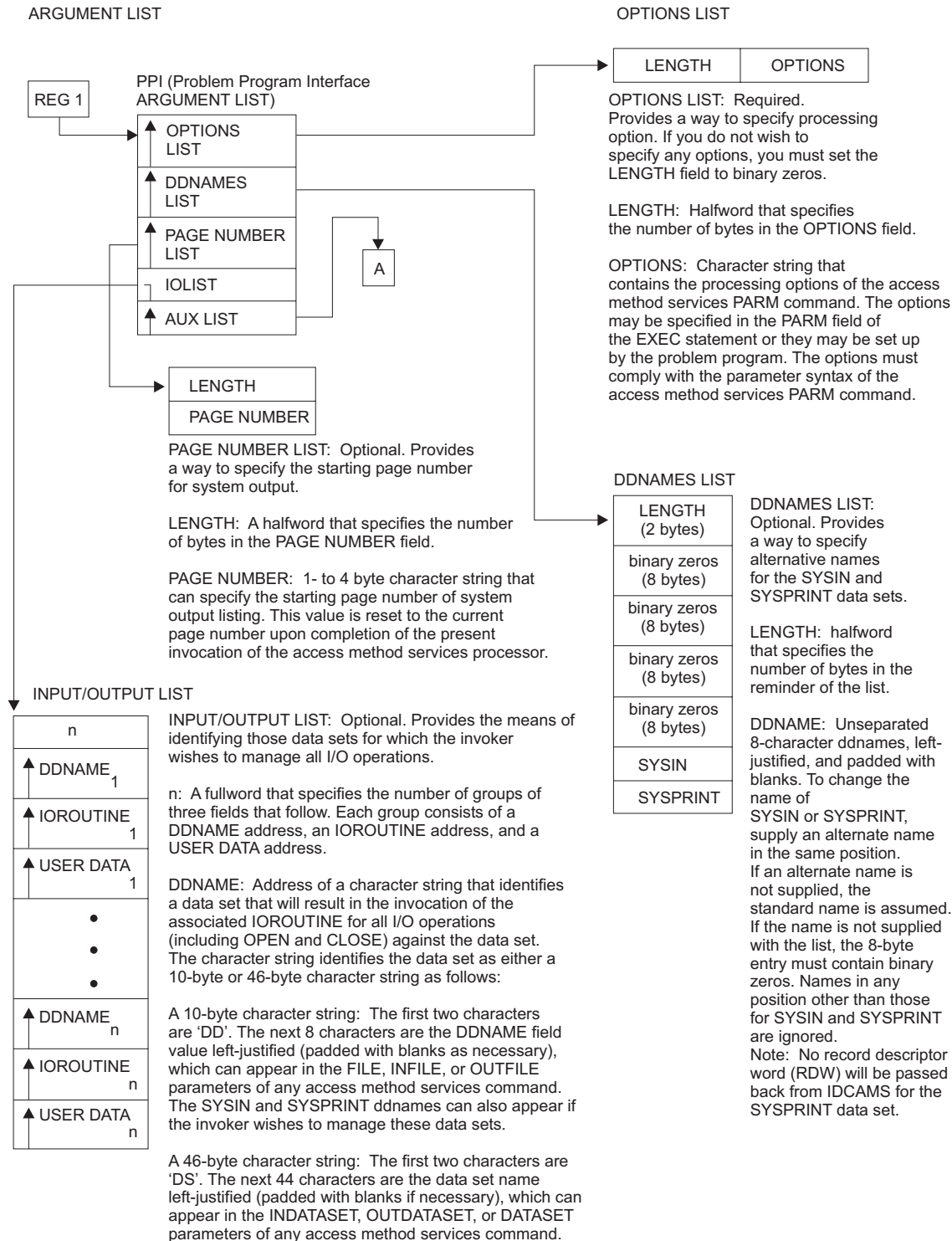
Figure 52. Processor Invocation Argument List from Your Program
