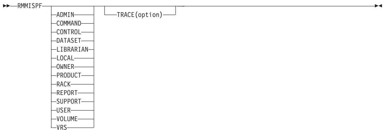
Figure 197. RMMISPF exec syntax diagram
