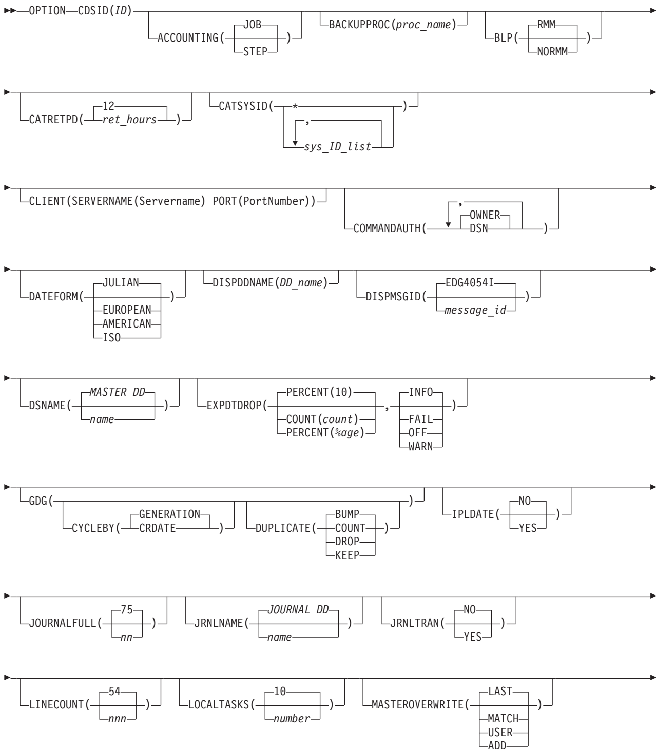
Figure 76. Parmlib member EDGRMMxx OPTION command syntax
