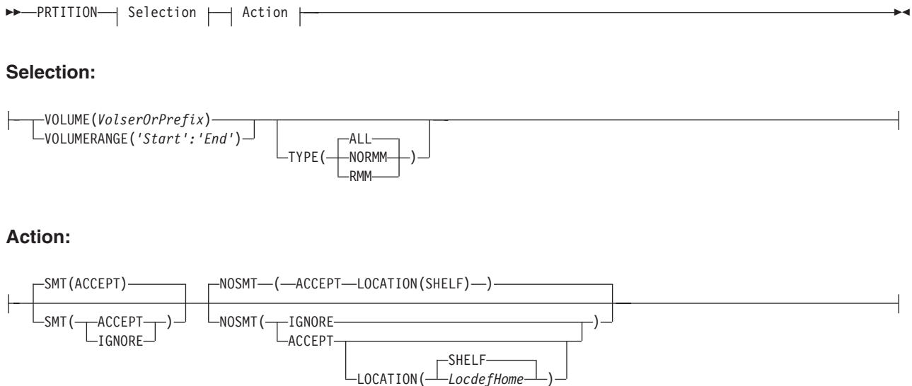
Figure 77. Parmlib member EDGRMMxx PRTITION command
