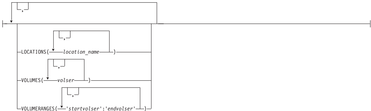
Figure 166. EDGUTIL SYSIN file
