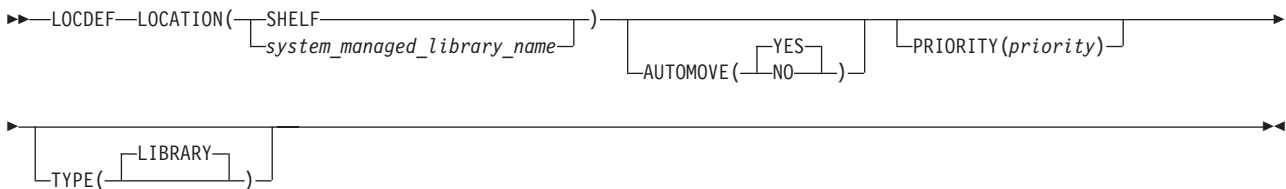
Figure 68. Parmlib member EDGRMMxx LOCDEF command for defining shelf and system-managed libraries
