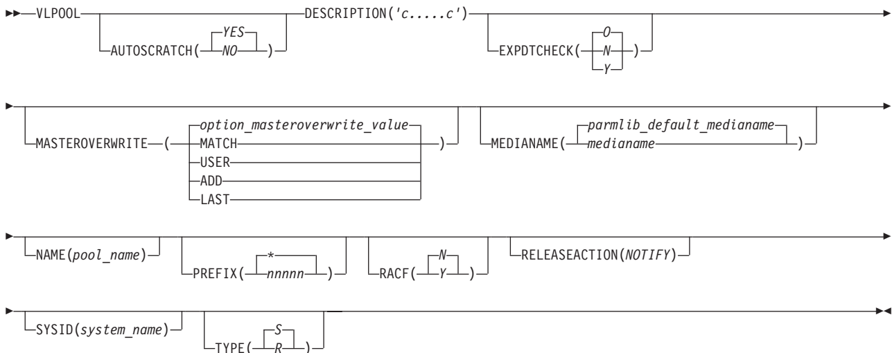
Figure 87. Parmlib member EDGRMMxx VLPOOL command syntax
