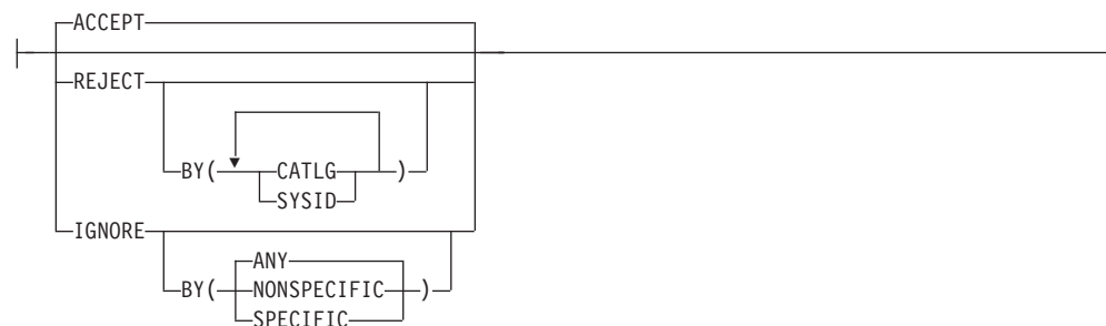
Figure 74. Parmlib member EDGRMMxx OPENRULE command
