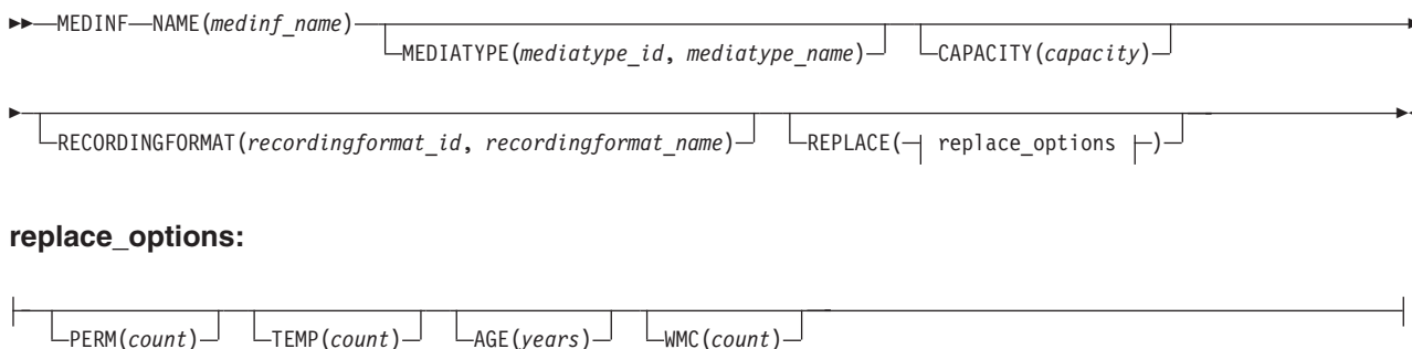
Figure 71. Parmlib member EDGRMMxx MEDINF command syntax
