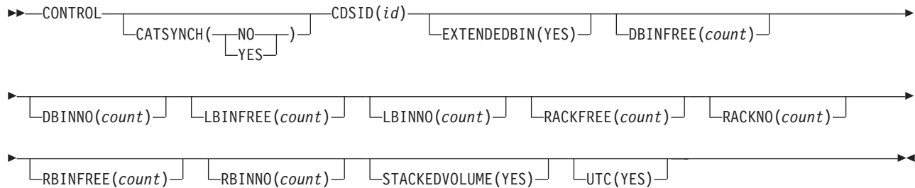
Figure 167. EDGUTIL SYSIN commands
