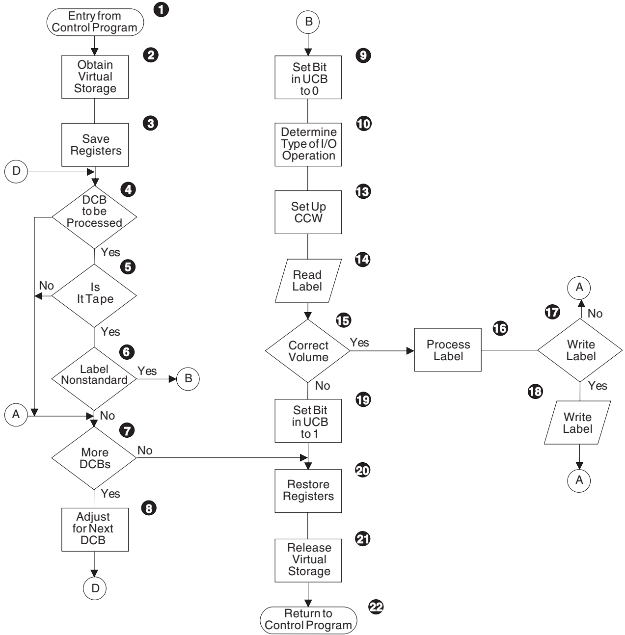
Figure 34. General Flow of a Nonstandard Label Processing Routine After Receiving Control from the Open Routine.
