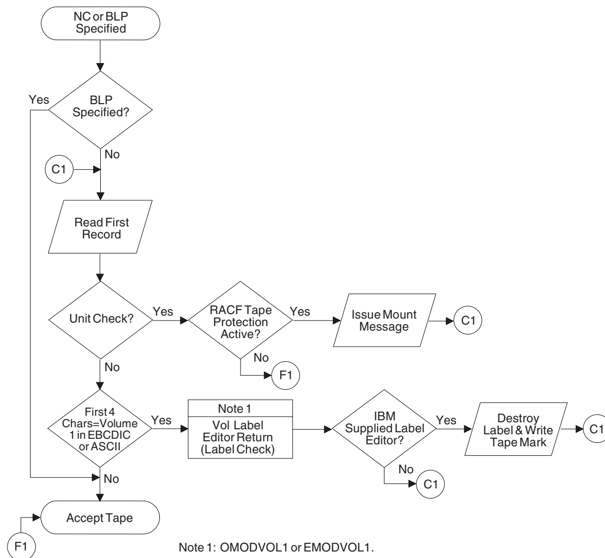
Figure 40. Verification of First Record When Unlabeled Tape Is Specified
