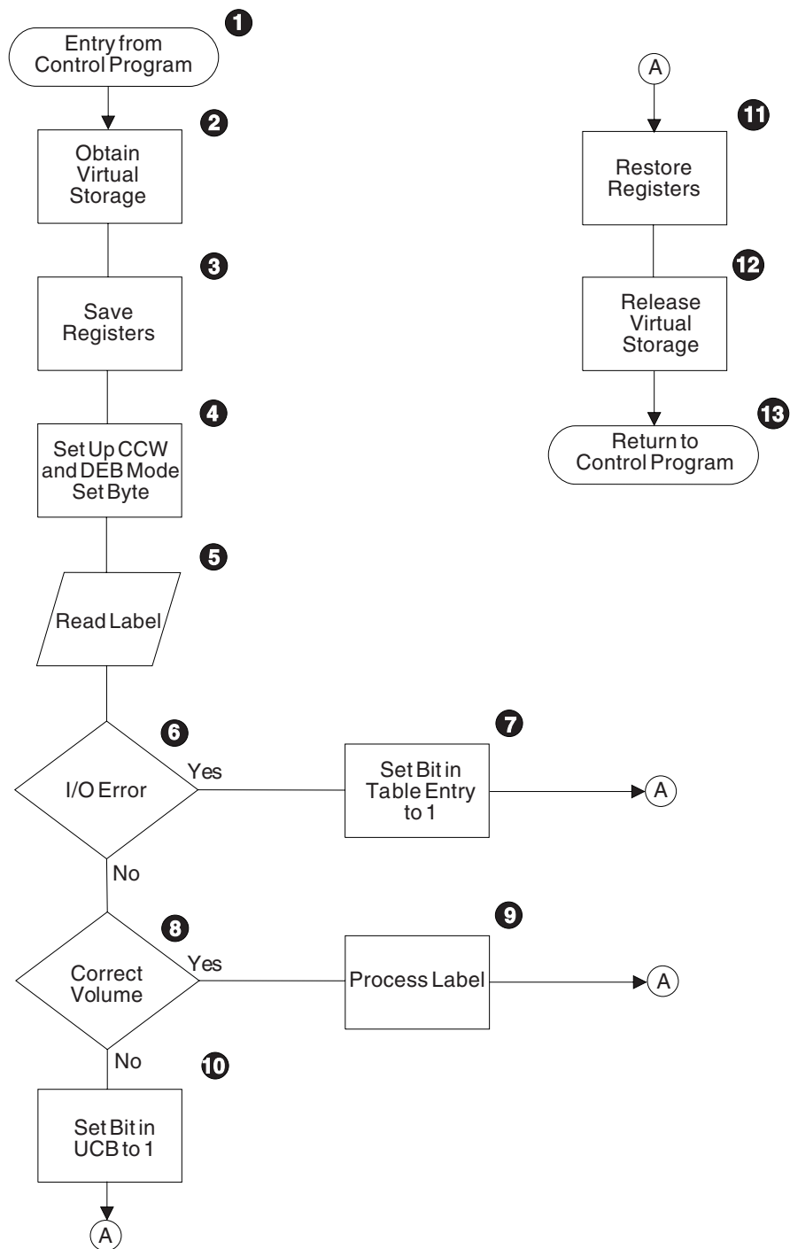
Figure 37. General Flow of a Nonstandard Label Processing Routine After Receiving Control from the Restart Routine
