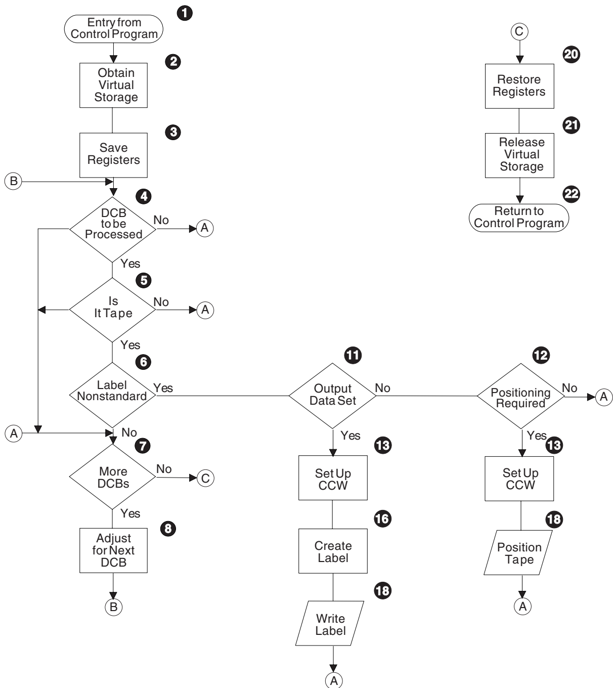
Figure 35. General Flow of a Nonstandard Label Processing Routine After Receiving Control from the Close Routine
