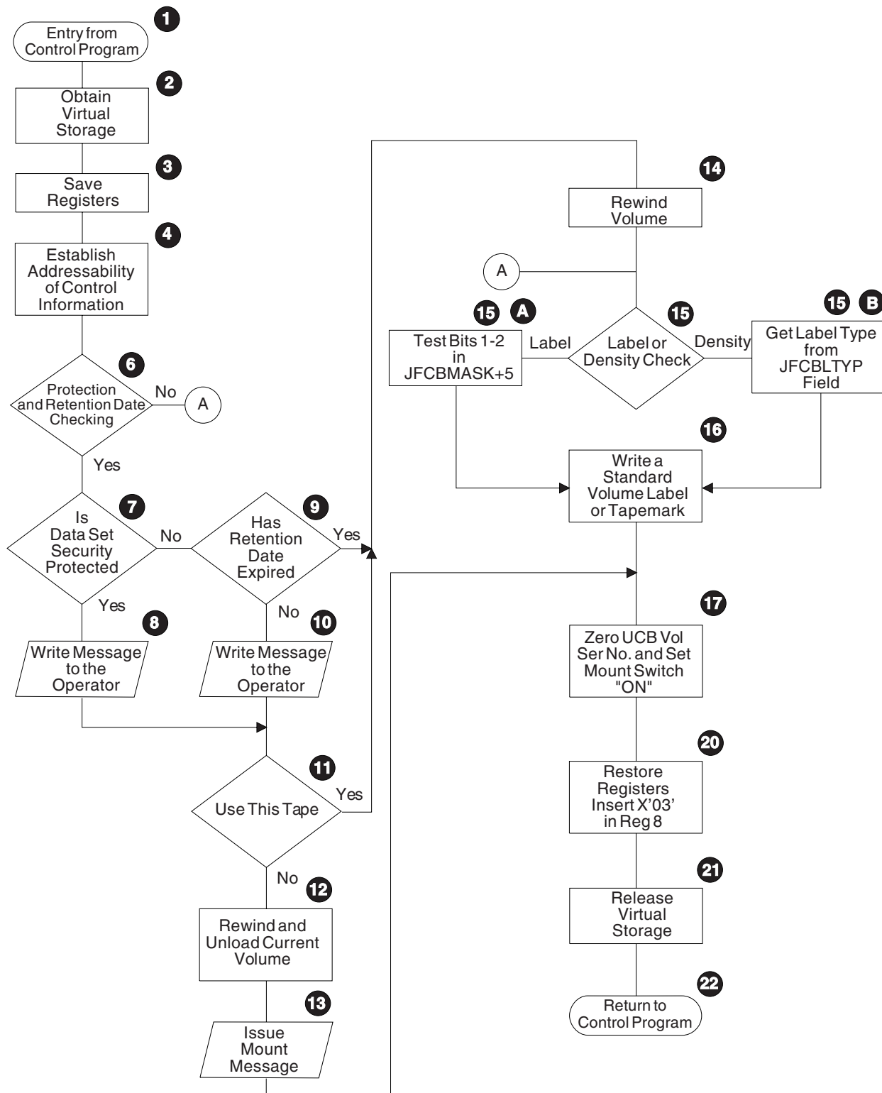
Figure 42. General Flow of an Editor Routine after Receiving Control from the EOVRoutine
