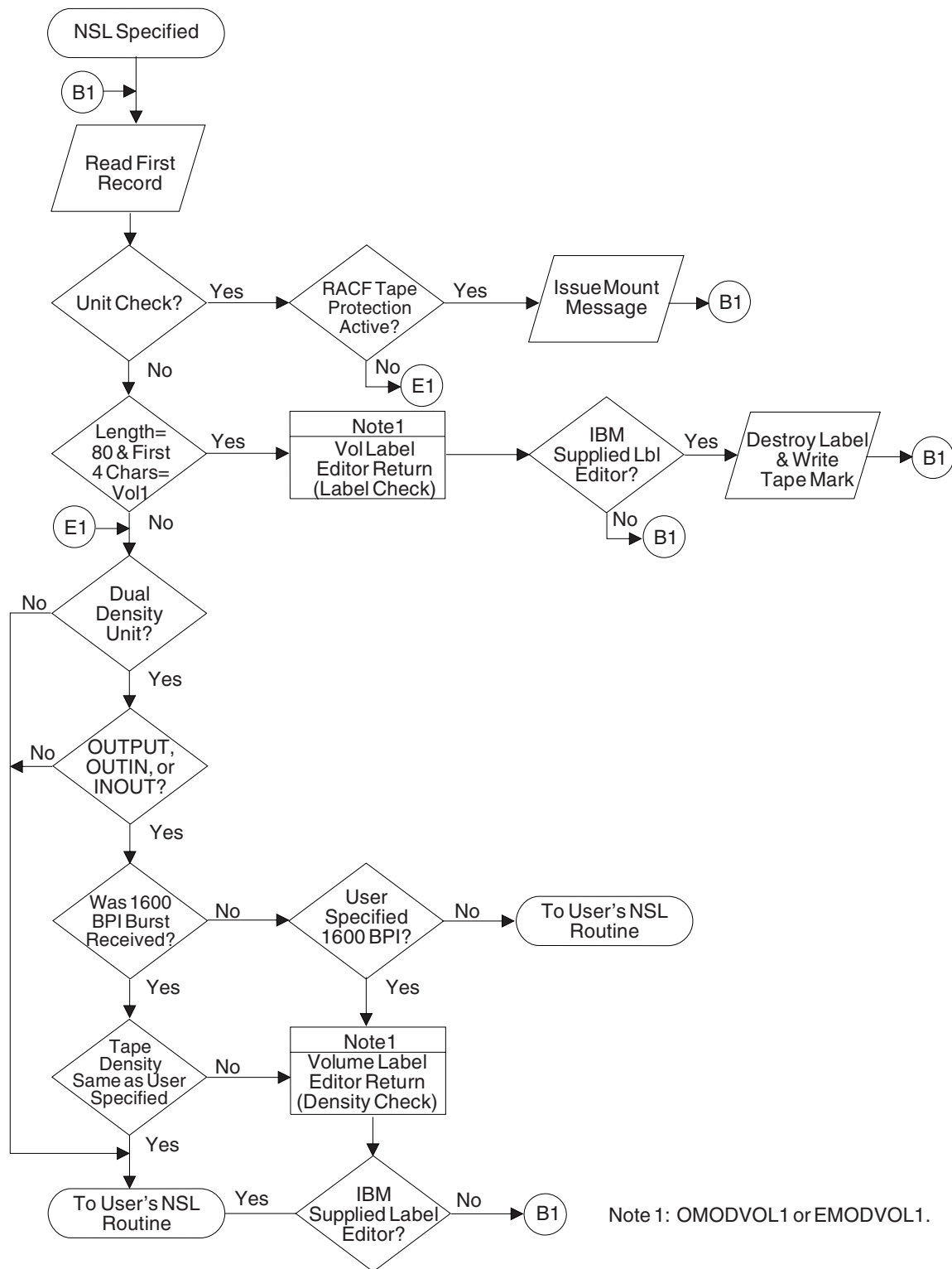
Figure 39. Verification of First Record When Nonstandard Labels Are Specified
