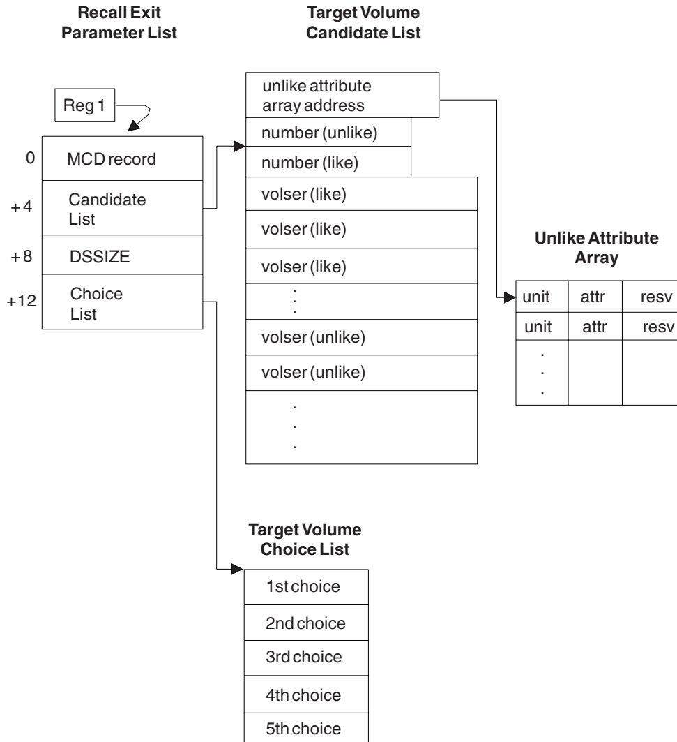
Figure 48. Recall Target Volume Data Structures
