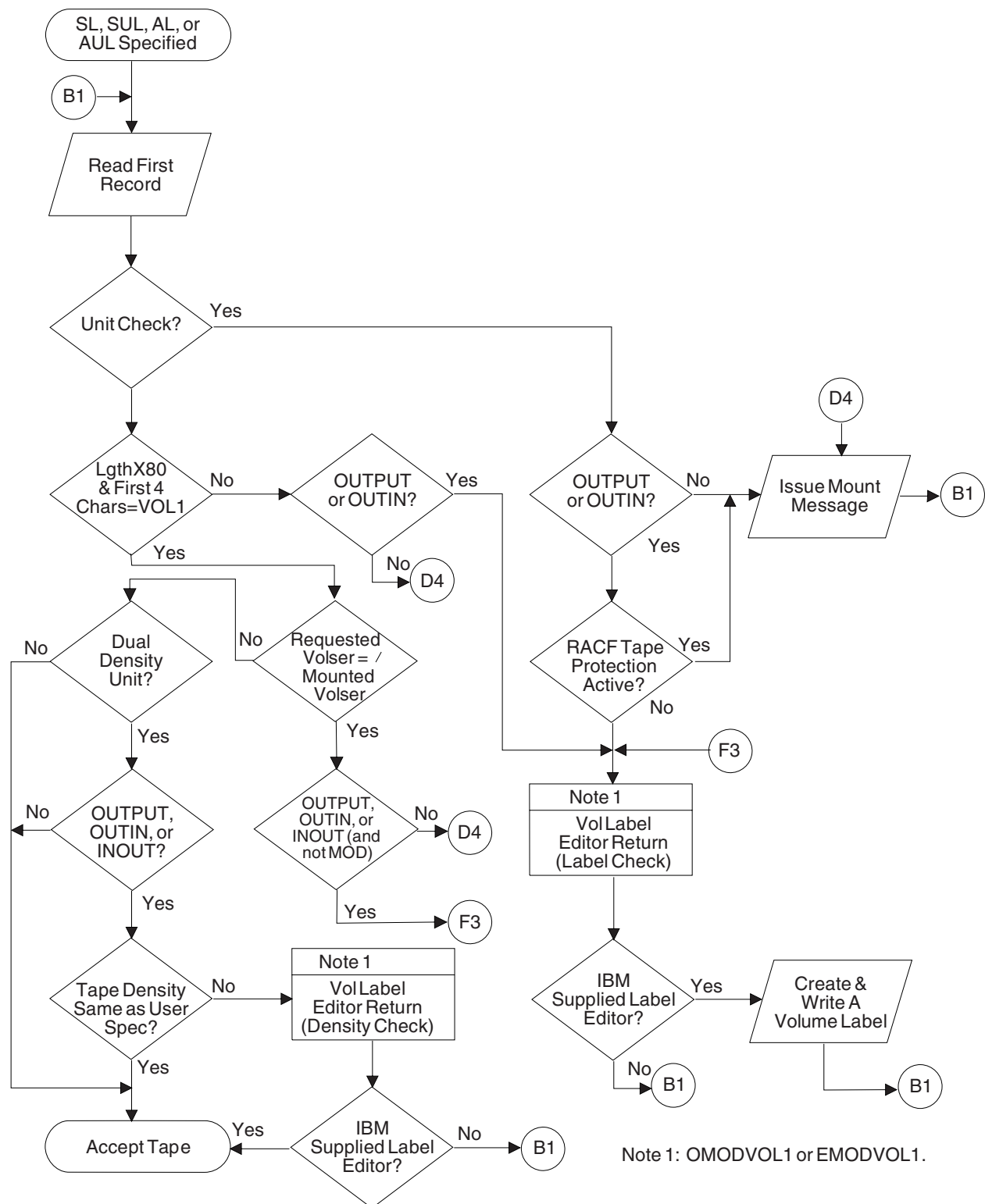
Figure 38. Verification of First Record When Standard Labels Are Specified
