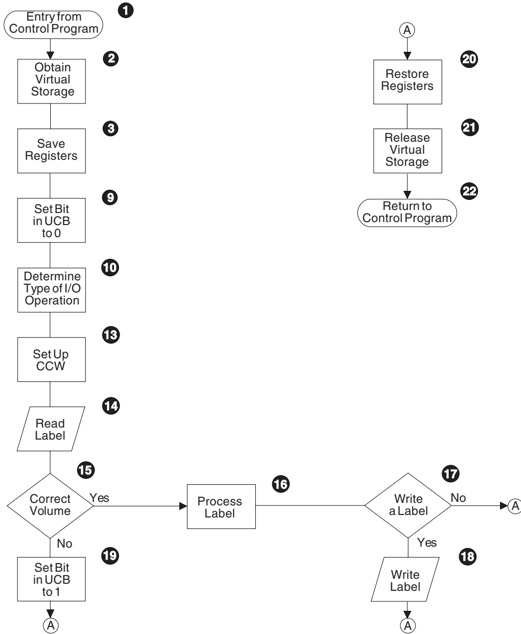
Figure 36. General Flow of a Nonstandard Label Processing Routine After Receiving Control from the EOVRoutine
