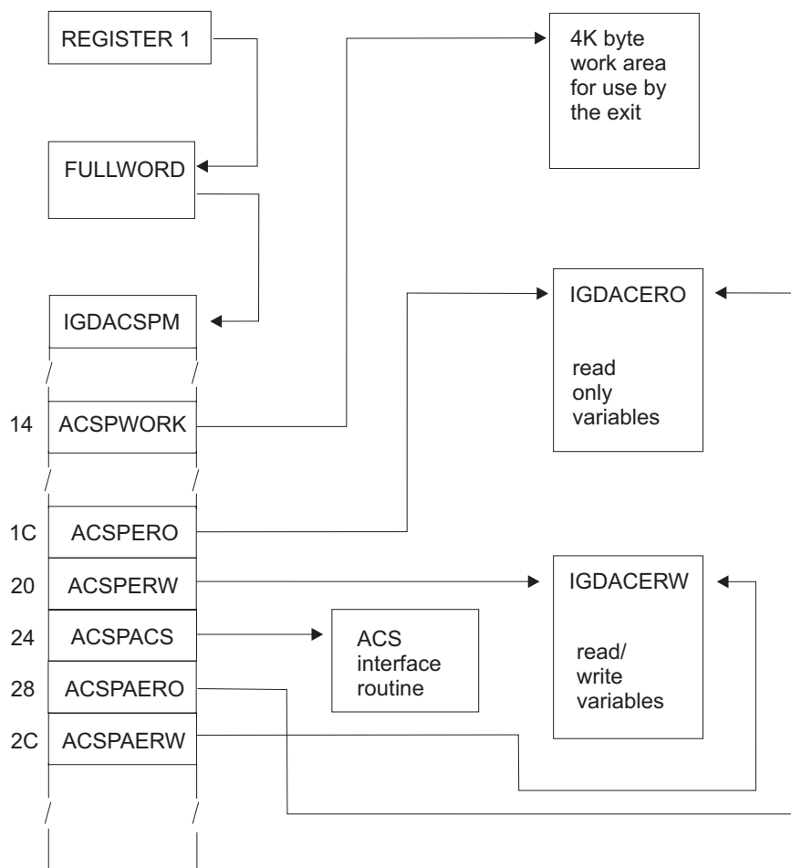
Figure 43. Parameter Structure for the ACS Installation Exits. This figure shows the control block structure upon entry into the exit. All offsets are in hexadecimal.
