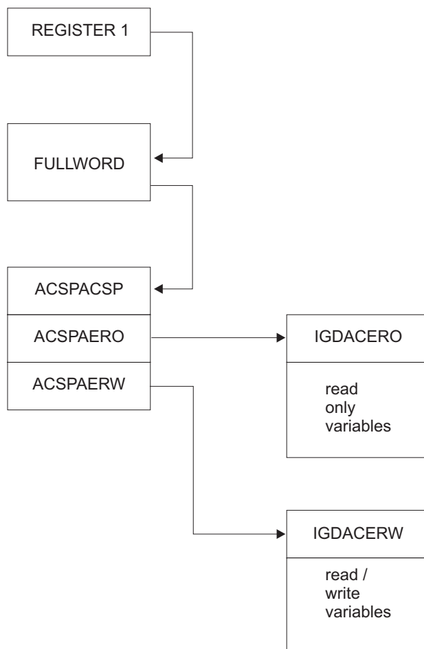
Figure 44. Parameter Structure for the ACS Interface Routine. This figure shows the control block structure for calling the ACS interface routine from the installation exit.
