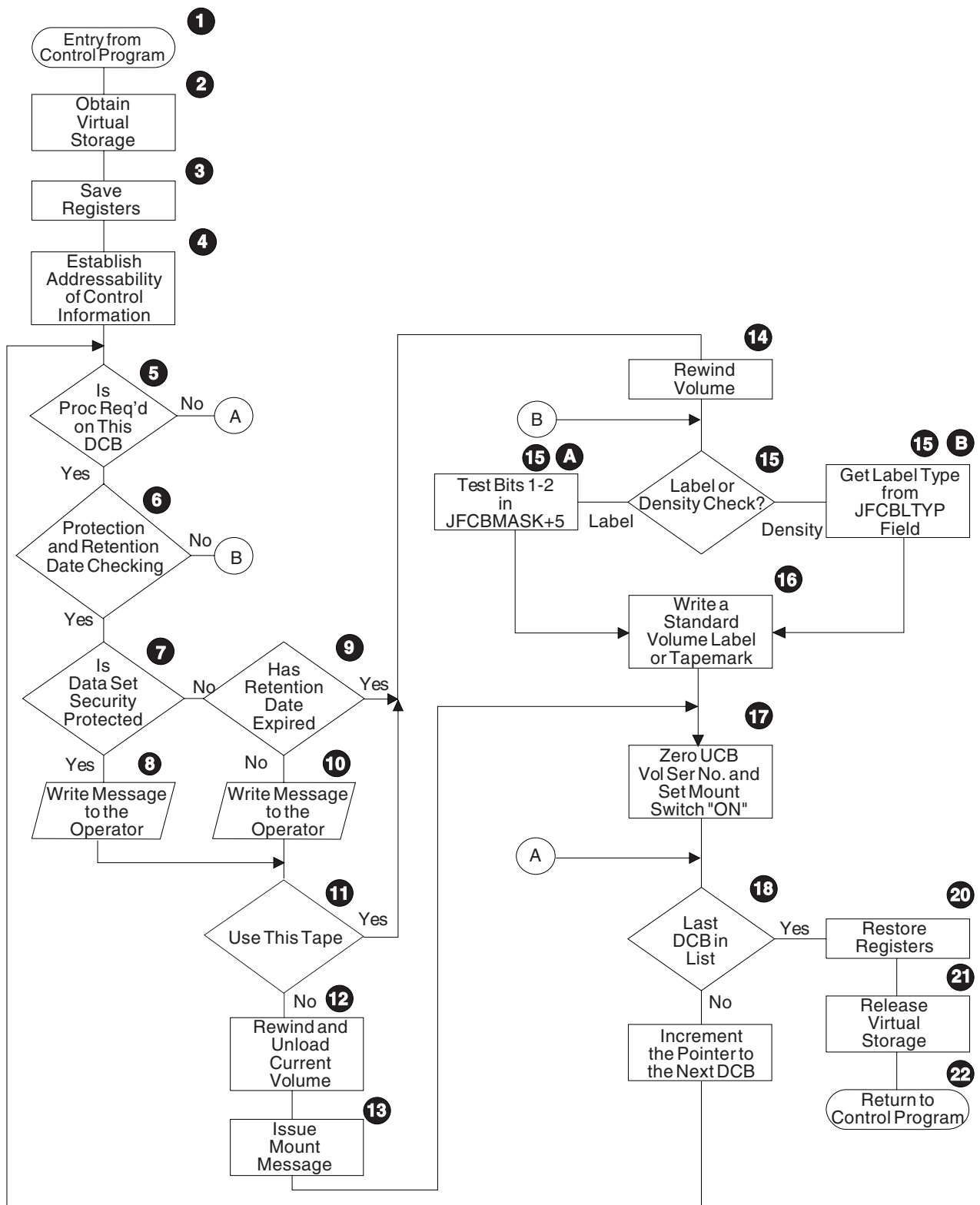
Figure 41. General Flow of an Editor Routine after Receiving Control from the Open Routine
