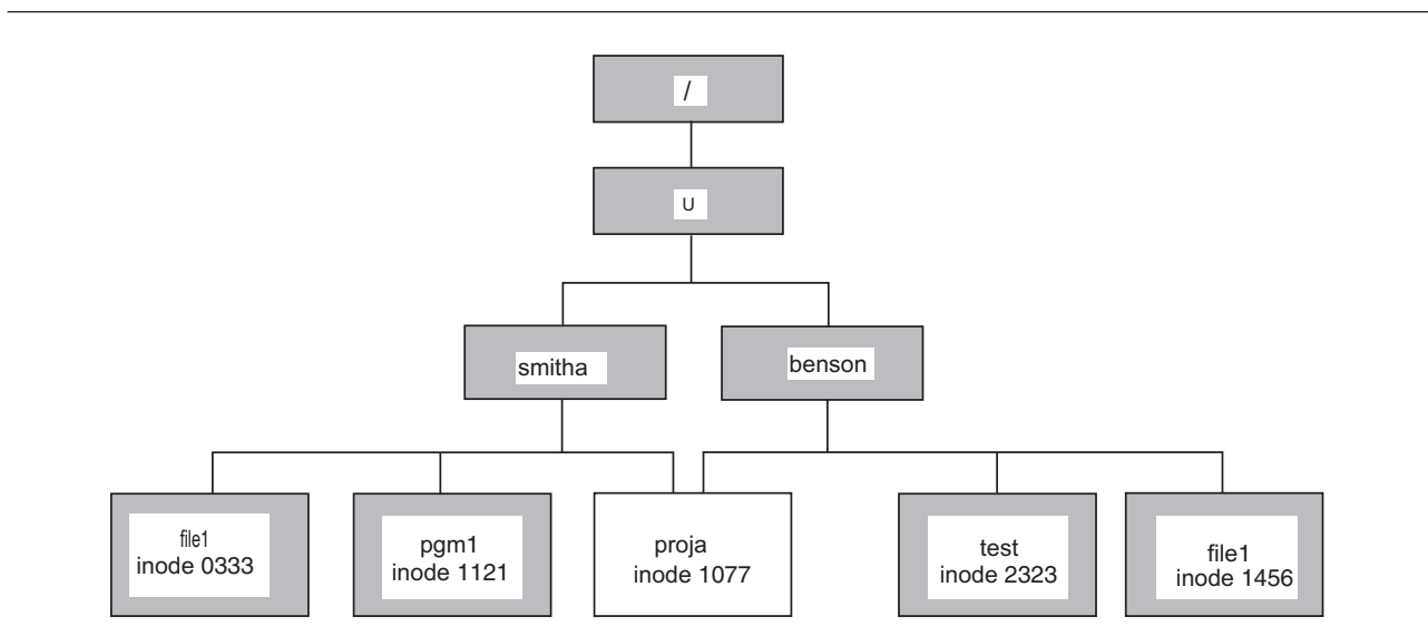
Figure 20. Hard link: a new name for an existing file. The hard link has an identical inode number.
