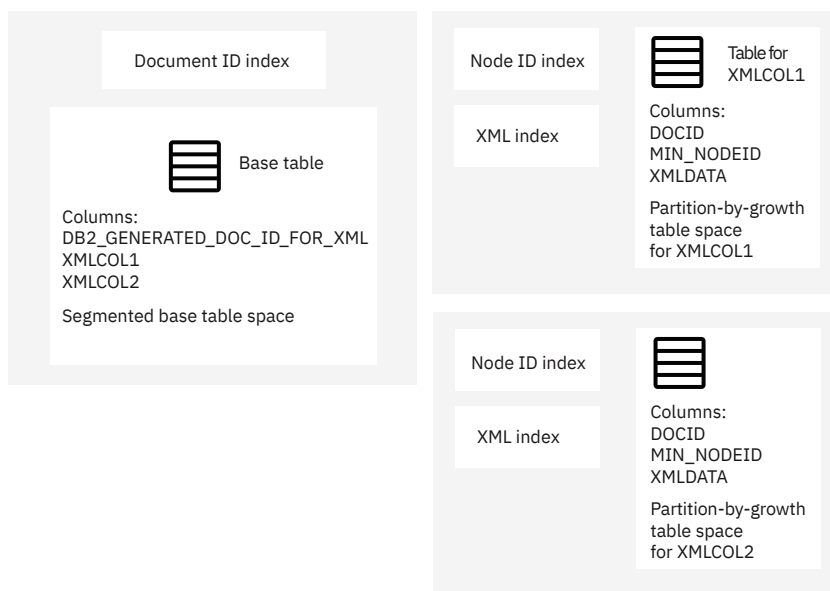
Figure 2. XML storage structure for a base table in a segmented table space
