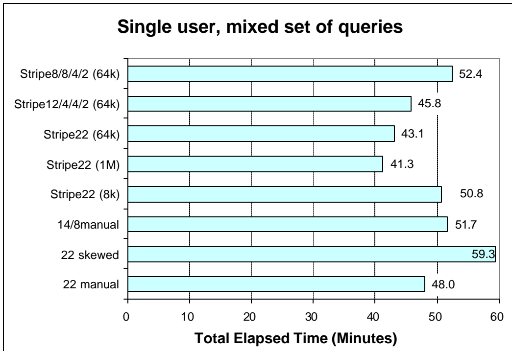
Figure 4: Total run times for a mixed set of queries
