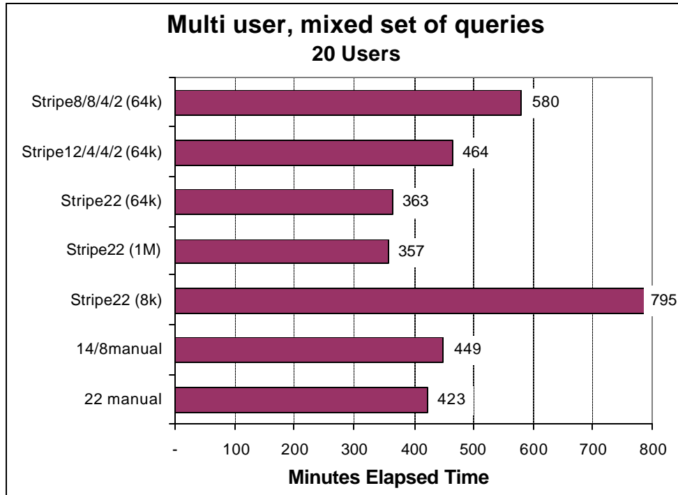
Figure 6: Total time for all 50 users running a mixed query workload
