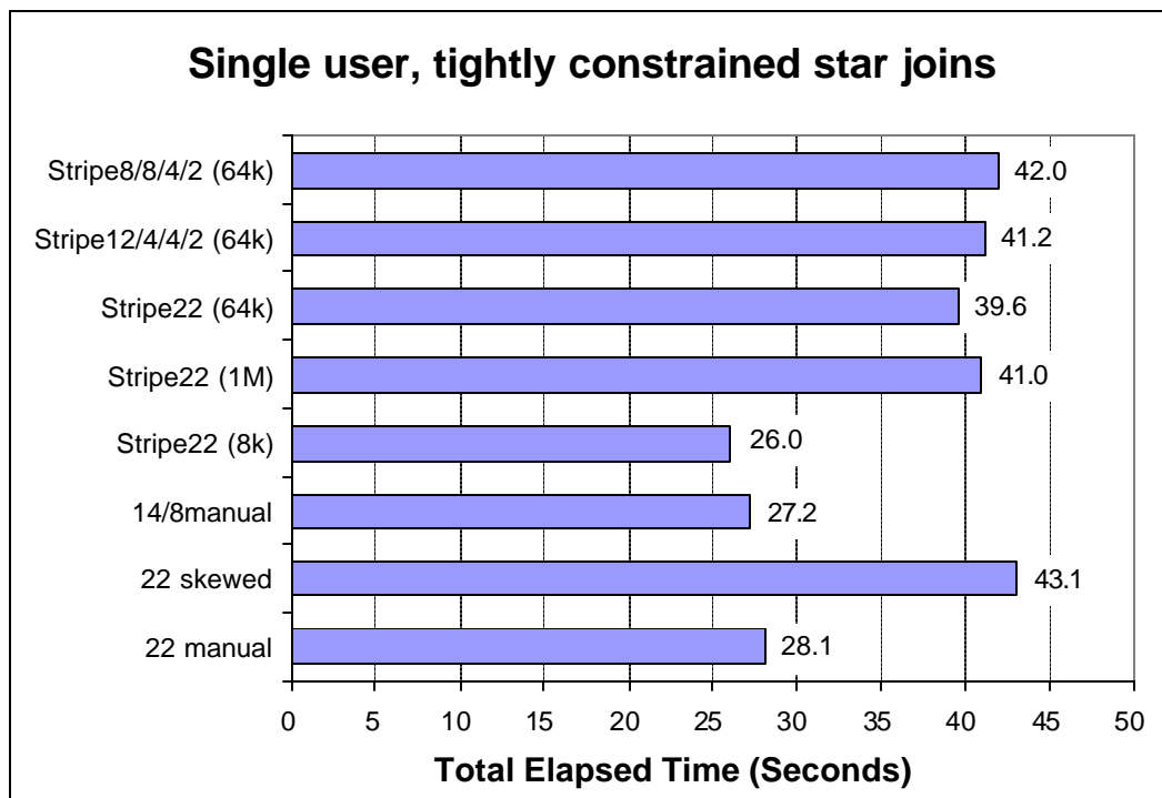
Figure 3: Total run times for a set of tightly constrained star join queries
