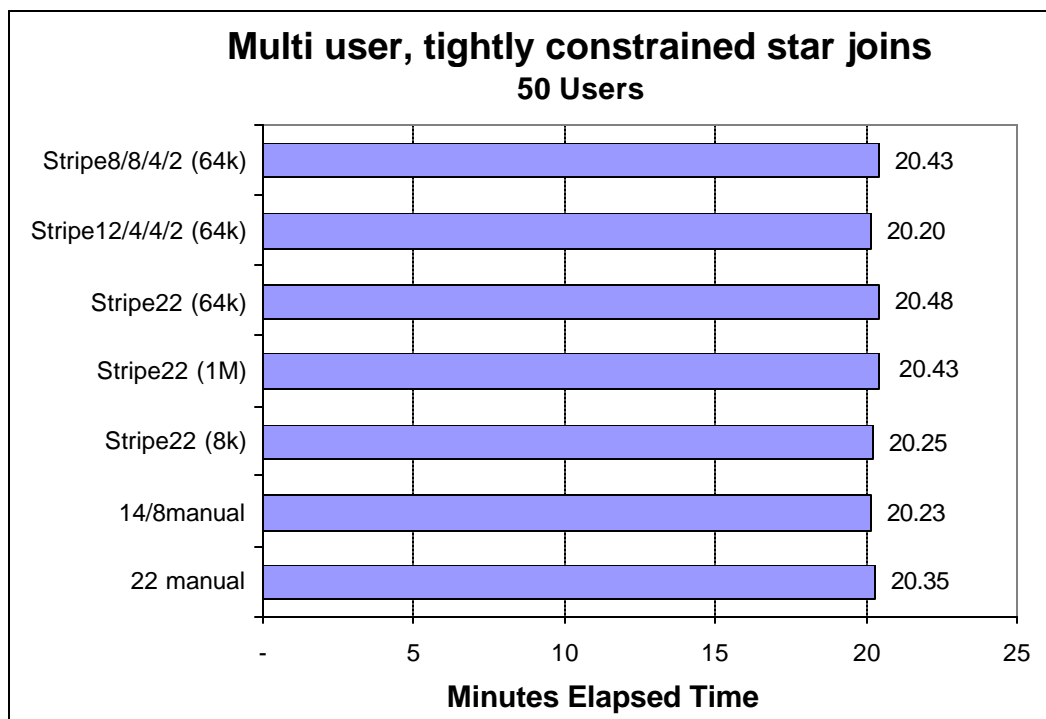
Figure 5: Total time for all 50 users to complete the workload
