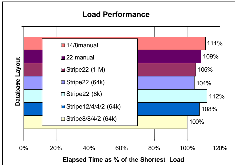
Figure 2: Load Performance for different storage layouts
