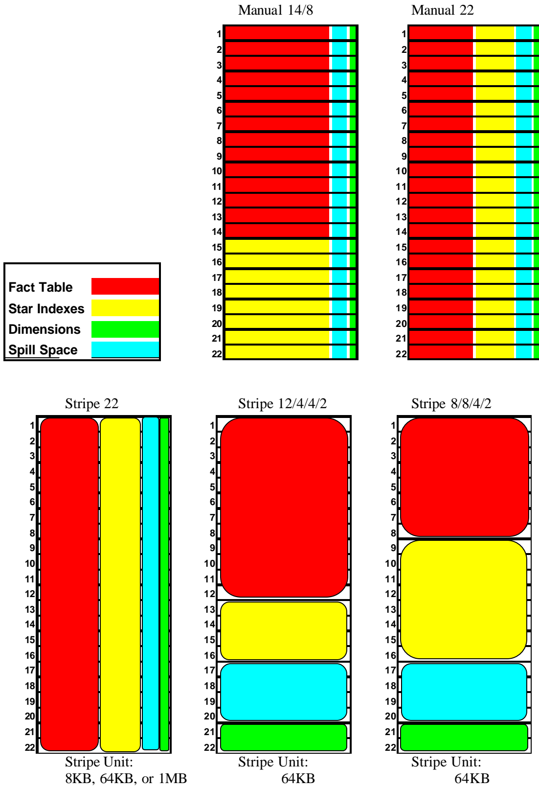
Figure 1: Storage Layout Alternatives
