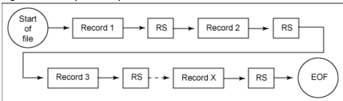
Figure 1. AWK input data split into records
